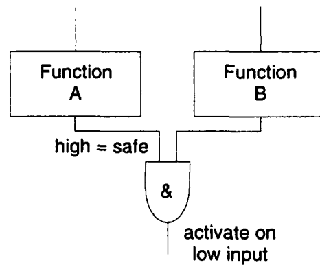
d. Functional Redundancy
