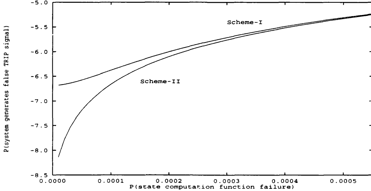
Figure B.6: Probability of Type-2 Failure as a Function of Software Failure
