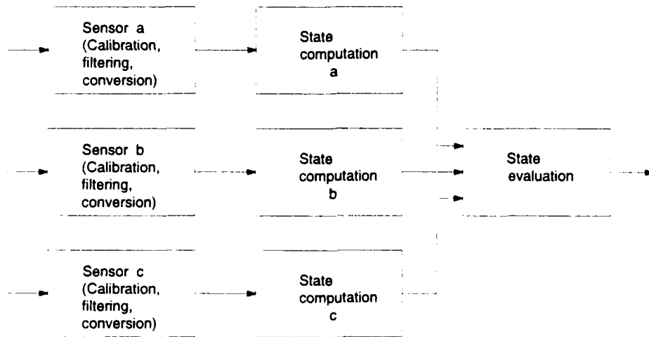
Figure B.4: Software Structure for Scheme I
