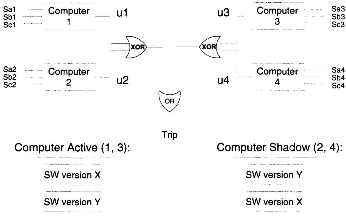
Figure B.7: Overview of the EDRB
