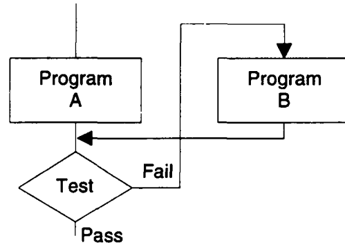
b. Recovery Block
