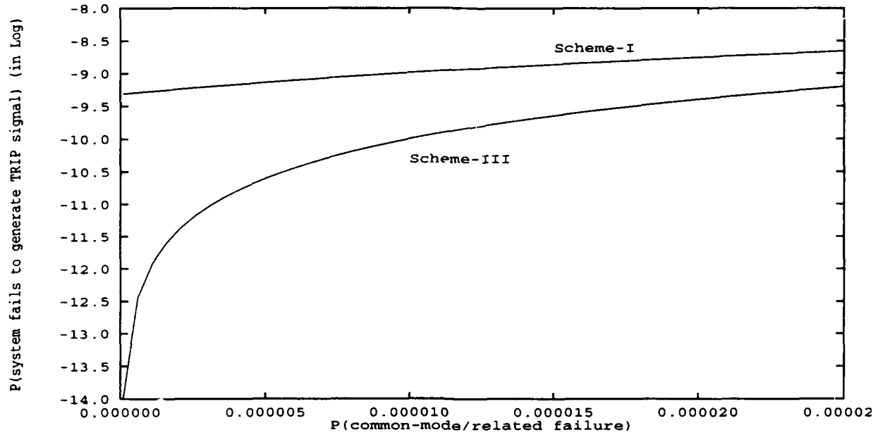
Figure B.13: Type-1 Failure Probability Improvement of Scheme III over Scheme I
