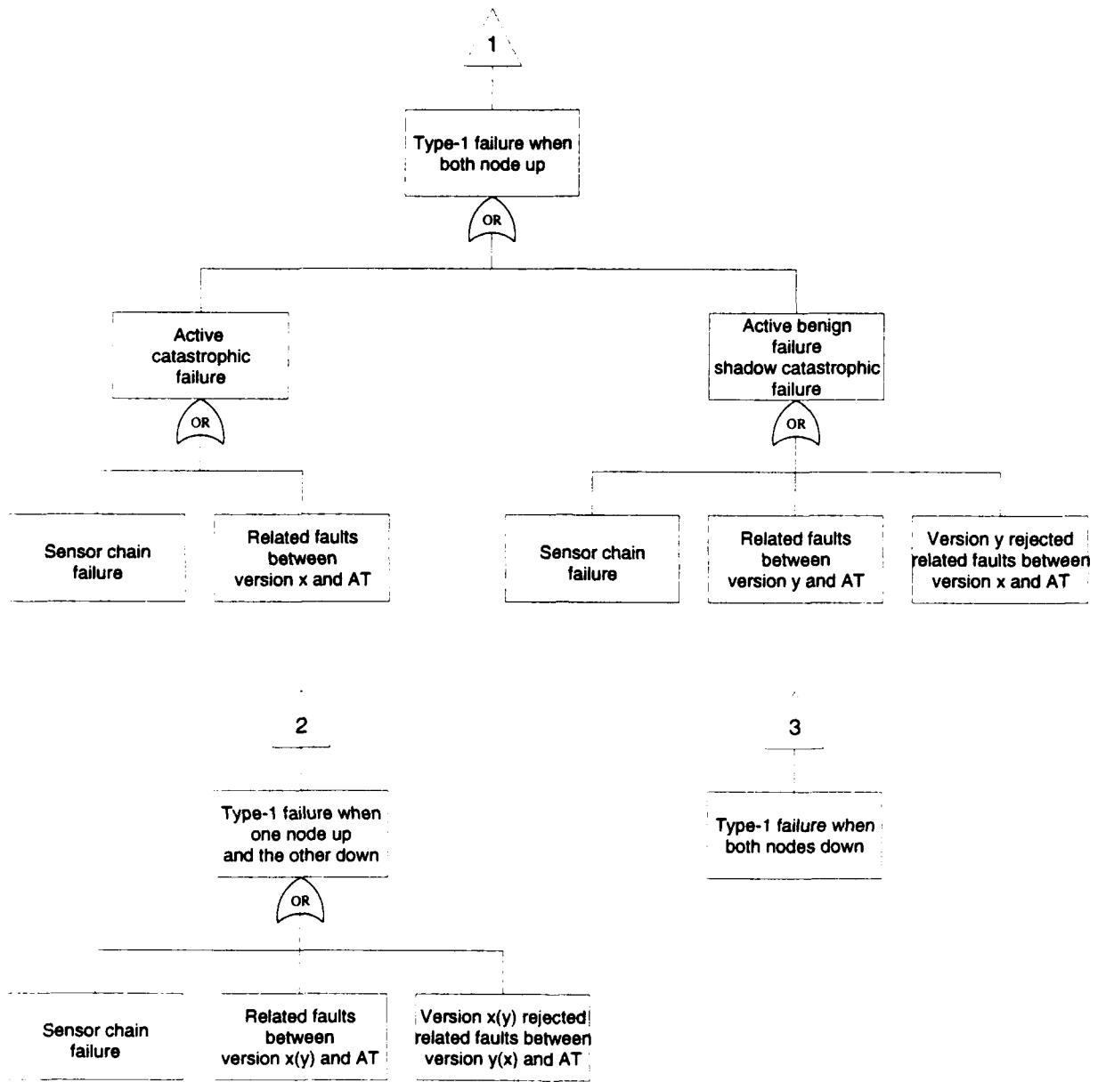
Figure B.11: Fault Tree for Type-1 Failure (II)
