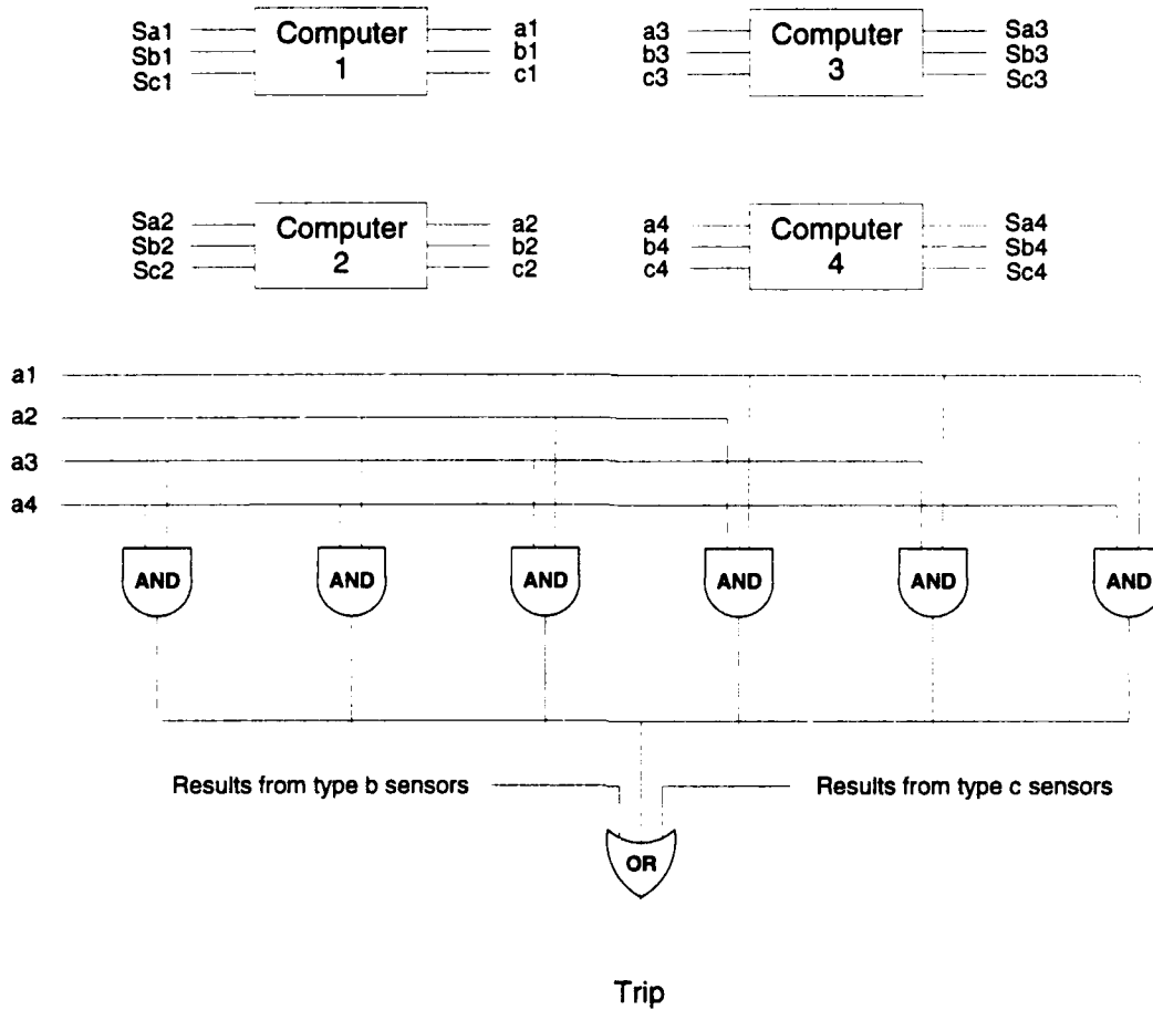
Figure B.3: Scheme II System for Generation of Trip Signal
