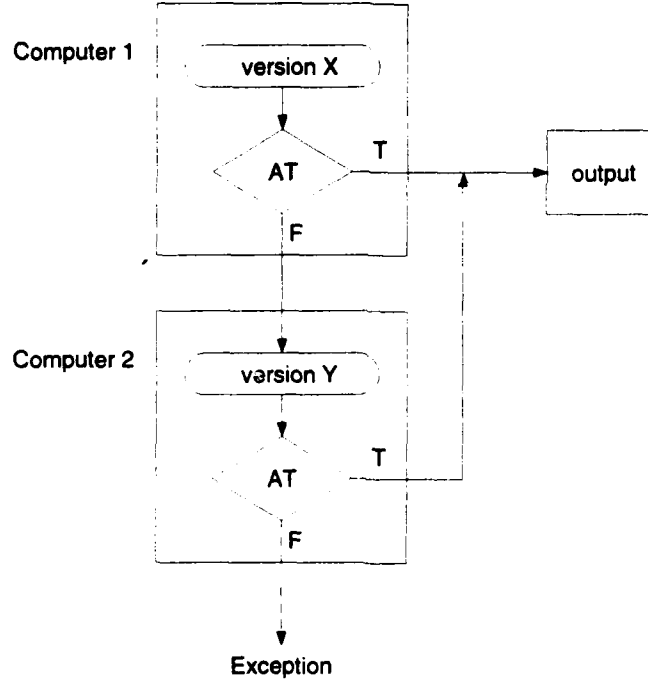
Figure B.8: EDRB Operation (high level)
