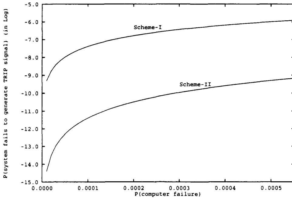
Figure B.5: Probability of Type-1 Failure as a Function of Hardware Failure
