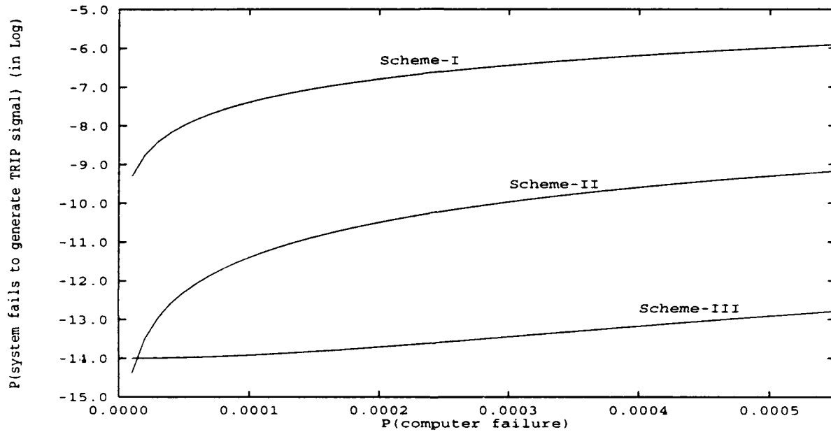
Figure B.12: Comparison of Scheme I, Scheme II and Scheme III
