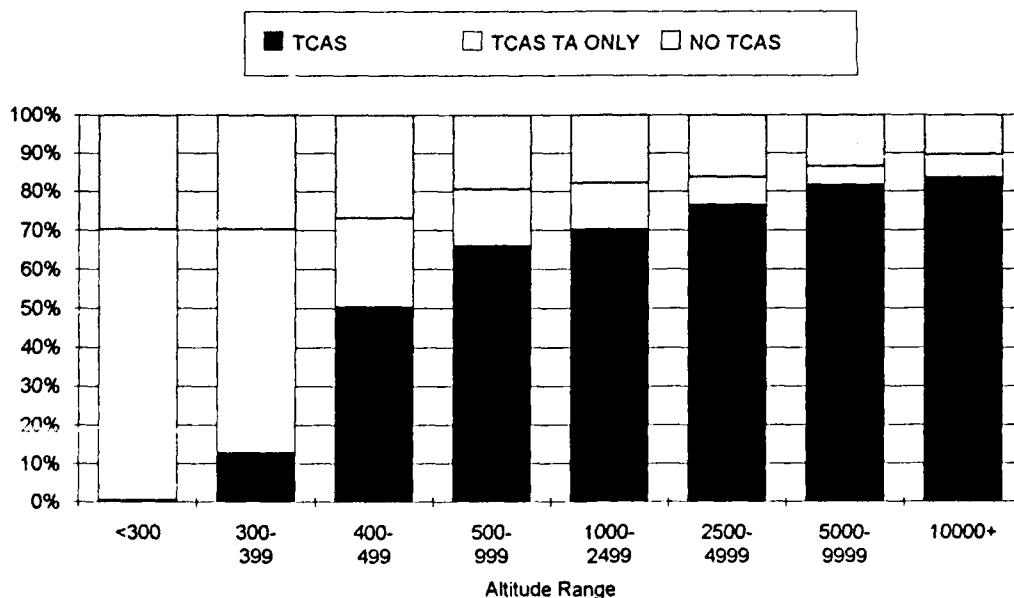
FIGURE 3. TCAS CAPABILITY REPORTED BY DOMESTIC MODE S EQUIPPED AIRCRAFT
