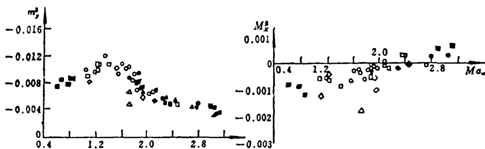
Fig. 8. Lateral-directional aerodynamic characteristics of X-15 craft [11]
