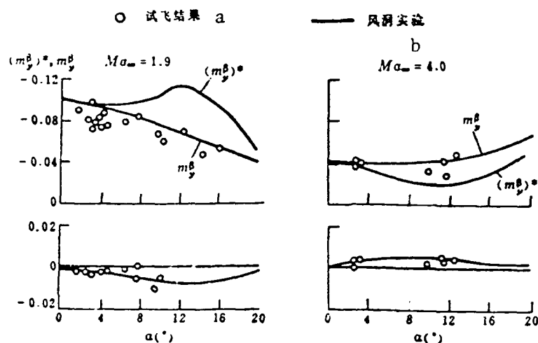
Fig. 9. Aerodynamic characteristics of X-15 craft
