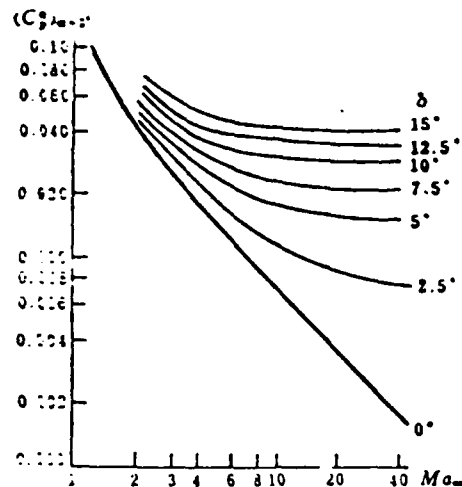
Fig. 10. Lift characteristics of single-wedge wing type
