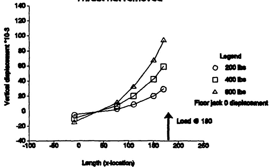
Figure 25. Gun tube load 180 inches from breech end of the gun tube.
