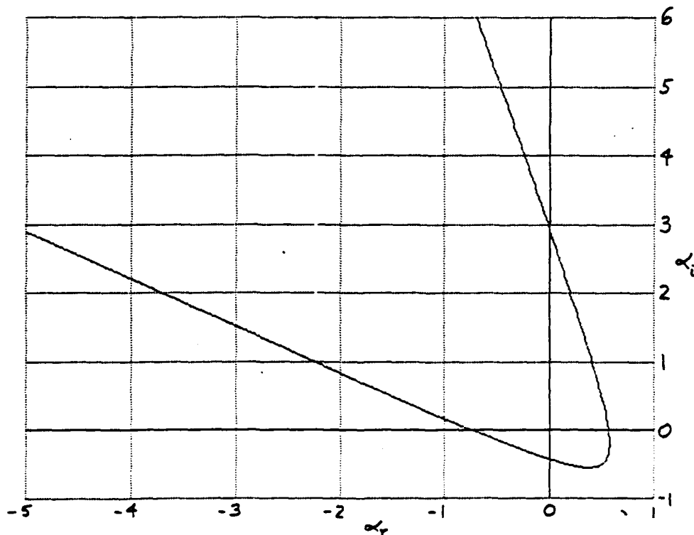
Figure 1. Region of Convergence of (59) for Example (78)
