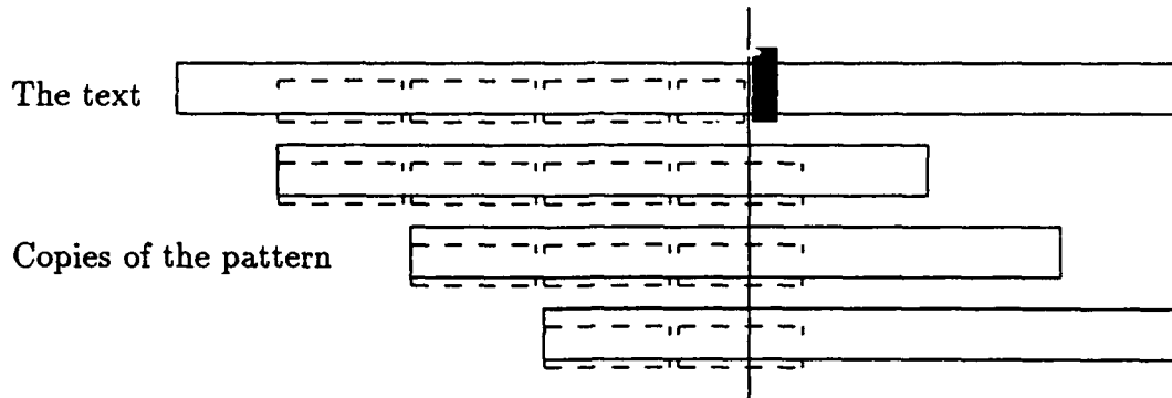
Figure 1: If \theta - q_i < \psi - 1 , then all pattern prefixes that start at text positions \{q_i\} terminate at the same text position.
