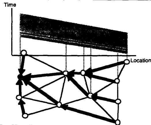
Figure 2: Green-band
