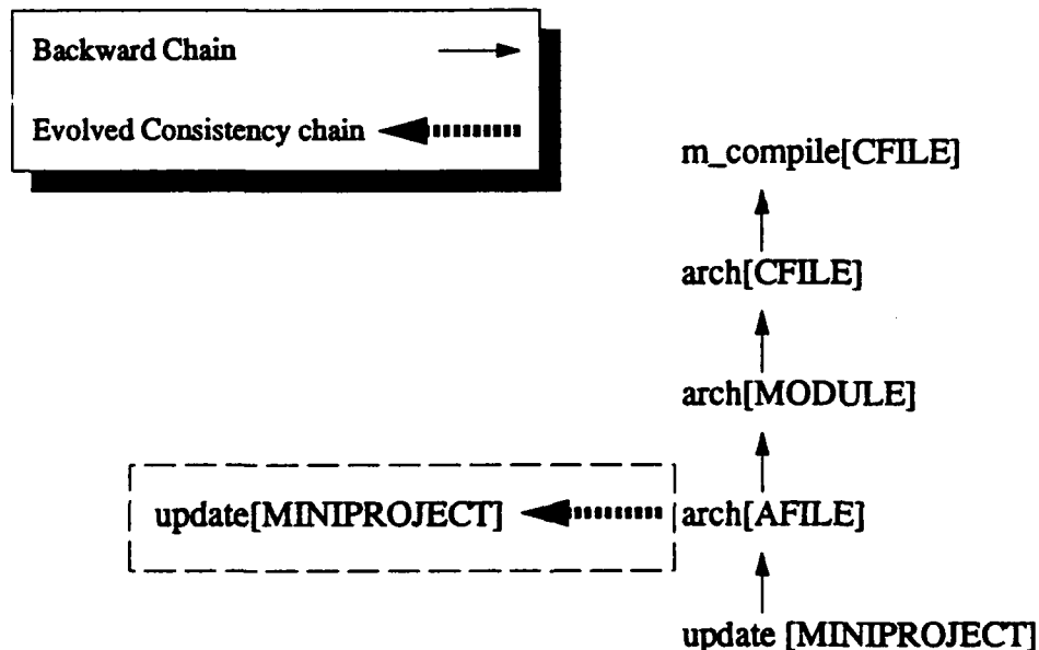
Figure 7-7: Subnetwork Containing update Rule
