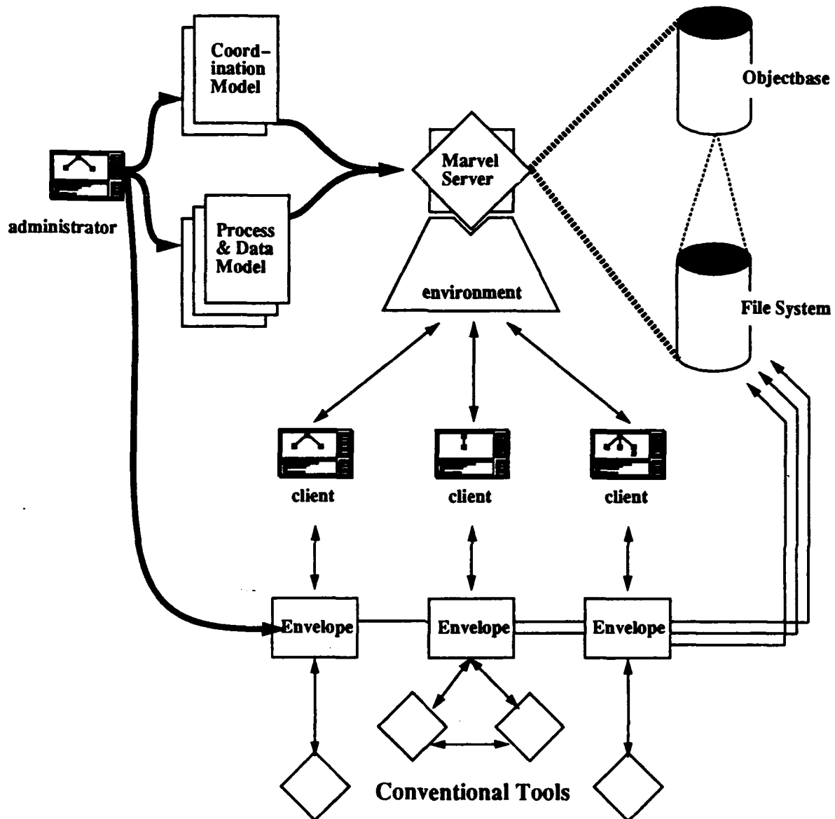
Figure I-1: Generic Marvel 3.1 Environment
