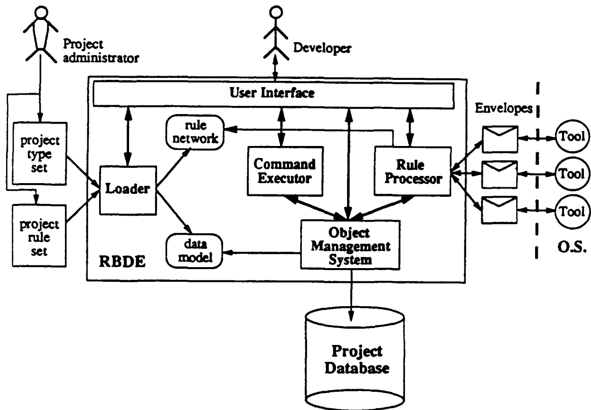
Figure 2-1: Overall System Architecture
