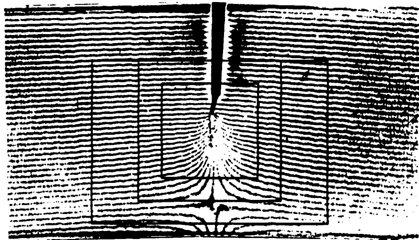
v-displacement field
