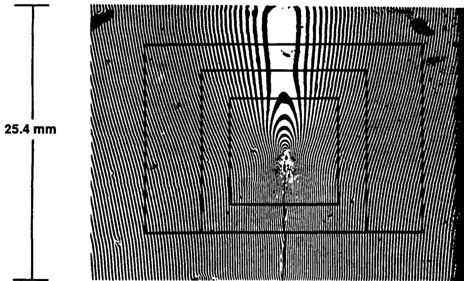
u-displacement field
