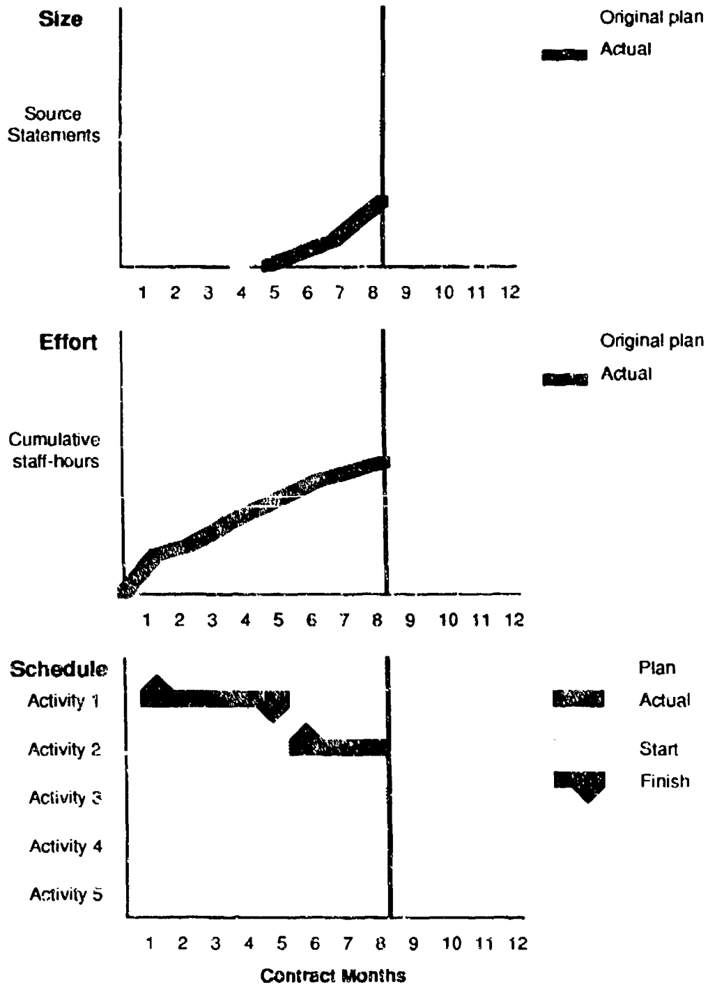
Figure 8. Example of Define Procedures Activity (4 of 5)
