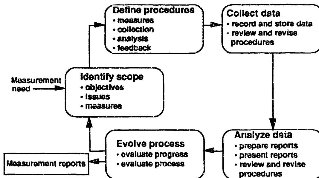
Figure 4. Measurement Architecture - Planning
