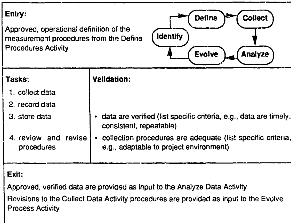
Figure 10. ETVX for Collect Data Activity
