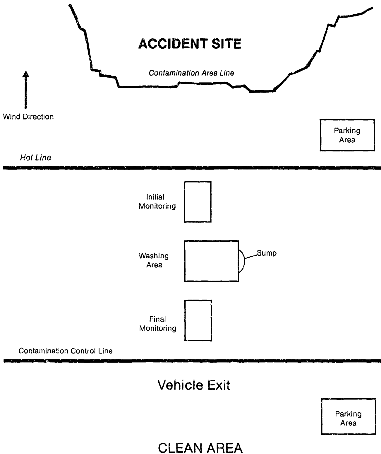
Figure 7-2. Vehicle Contamination Control Station Example.
