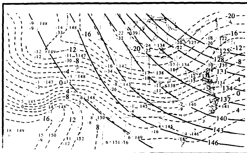
Figure 6. 850 mb analysis for 1200 UTC 7 March 1986. Dashed lines are isotherms analyzed every 2°C. Solid lines are isoheights analyzed every 3 dm.
