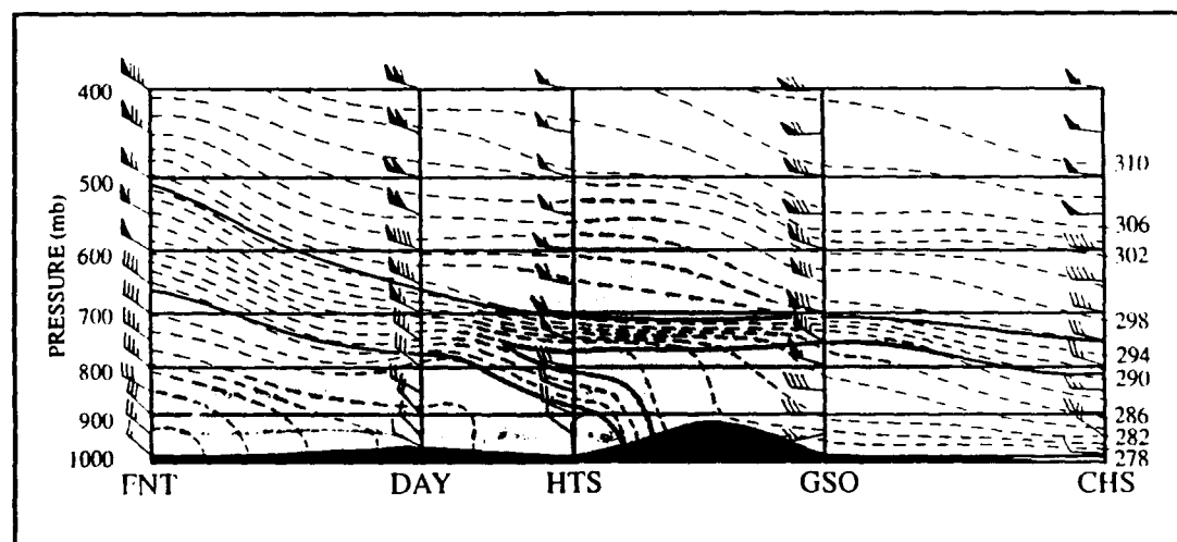
Figure 7. Vertical cross-section taken perpendicular to the front from Flint (FNT), Michigan to Charleston (CHS) South Carolina at 1200 UTC 7 March 1986. Dashed lines are isentropes analyzed every 2 K. Winds are plotted every 50 mb with full (half) barbs representing 5 \text{ m s}^{-1} ( 2.5 \text{ m s}^{-1} ). Flags represent 25 \text{ m s}^{-1} . Relative humidity of greater than 80% indicated by the shaded region in gray. Frontal zones marked with solid black lines.
