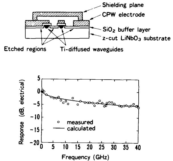
Figure 3. LiNbO 3 optical modulator with 40 GHz bandwidth [7].
