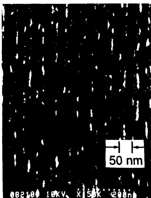
Fig. 1. Scanning electron micrograph of a MSMPD with 25 nm finger spacing and finger width. The metals are Ti and Au.
