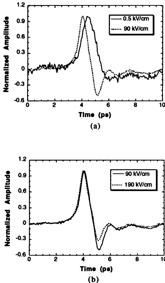
Figure 3. Comparison of the waveforms with normalization. (a) While the waveform at 0.5 kV/cm is unipolar, that at 90 kV/cm is bipolar, which indicates velocity overshoot. (b) The smaller negative peak at 190 kV/cm shows that the overshoot (deceleration of the carriers) decreases at very high fields.
