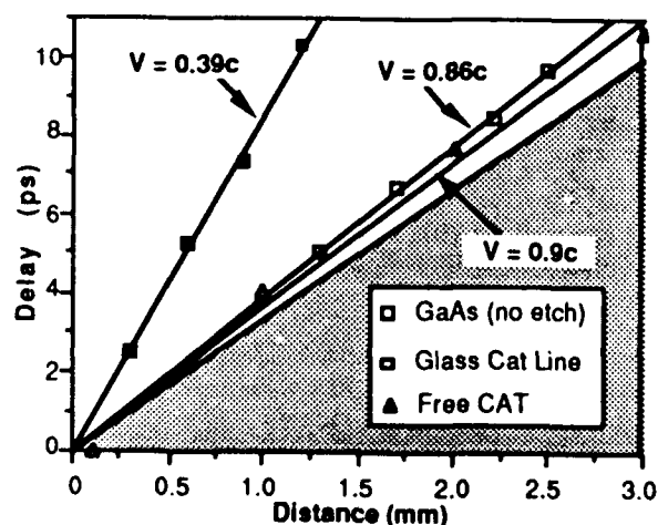
Fig. 5 Plot of delay (as measured by midpoint of linear fit to risetime) versus propagation distance. Free CAT corresponds to the geometry of Fig. 1. Velocity, v , is found from a linear fit to the data. Shaded area is bordered by v=c .
