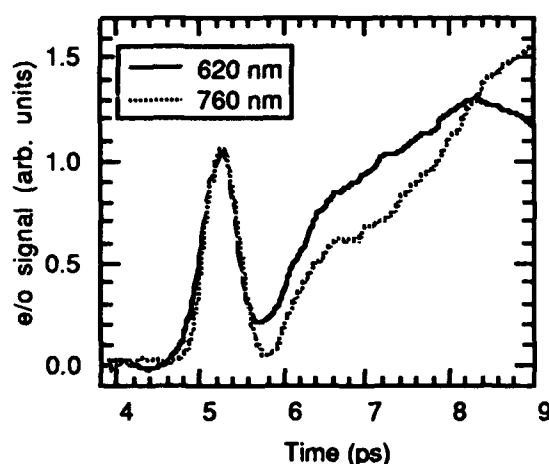
Figure 3. Comparison of electro-optically sampled data for SI GaAs taken at \lambda=620 nm (CPM) and 760 nm (Ti:Sapphire).
