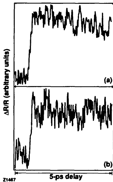
Figure 4. Normalized \Delta R/R measured with a 2-eV probe on the YBCO-II microbridge biased by the following levels of electric current: (a) 0 and (b) 15 mA. The critical current of the microbridge was 12 mA. The temperature was about 79 K and the pump intensity was \sim 40 \mu\text{J}/\text{cm}^2 .
