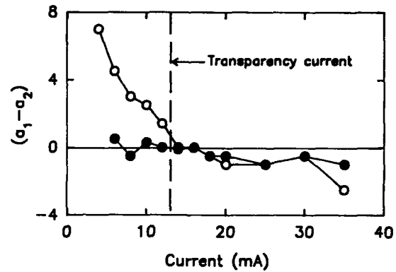
Figure 7. Magnitude of (a_1 - a_2) , the spectral-hole burning component of the system response function, as a function of bias current for co-polarized (open circles) and cross-polarized (solid circles) measurements.
