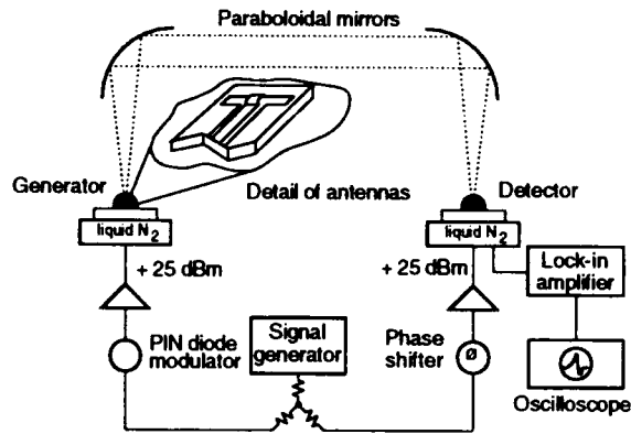
Figure 2. Diagram of THz signal generation/detection system. Inset shows detail of the magnetic dipole (slot) antennas.
