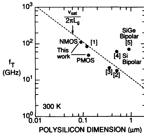
Figure 1. Cutoff frequency, f_T versus gate length for NMOS field effect transistors [1-3] or emitter width for Si-based bipolar transistors [4,5]. The dashed line estimates f_T \approx v_{sat}/2\pi L_g for NMOS devices, where L_g is the gate length and v_{sat} is the electron saturation velocity ( \sim 7 \times 10^6 \text{ cm/sec} at room temperature).
