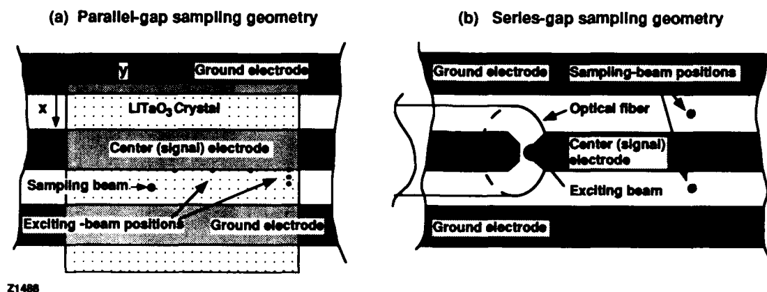
Figure 1. A schematic representation of the sampling geometries employed. (a) The parallel-gap geometry, with both excitation and sampling beams focused through an electro-optic \text{LiTaO}_3 crystal and (b) The series-gap sampling geometry, with the excitation beam guided through an optical fiber.
