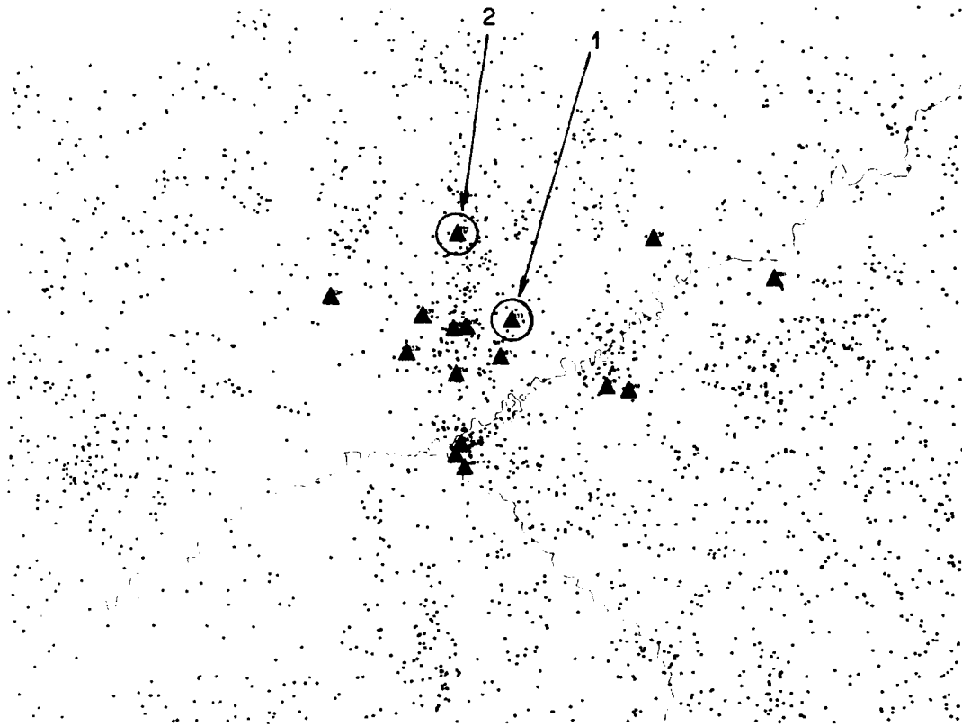
Figure 6.5: Lightning strike map of study area up to 30 days after Julian day 166.
