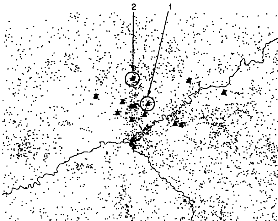
Figure 6.4: Lightning strike map of study area after Julian day 166.
