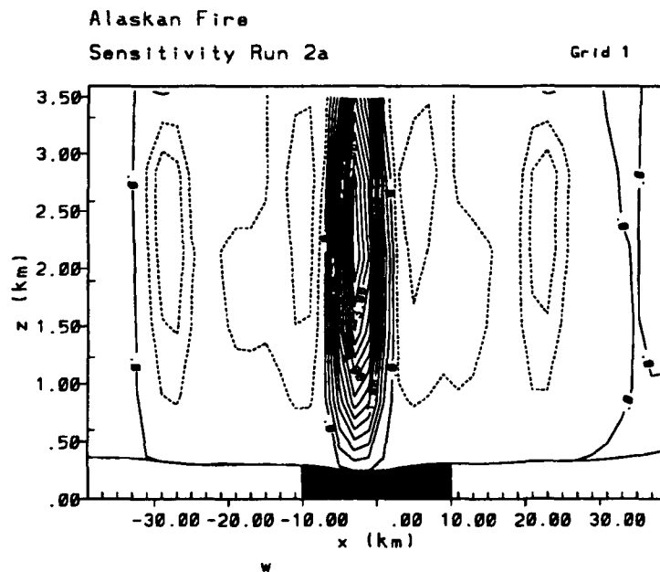
Figure 5.9: Vertical velocity field ( w ) in \text{cm s}^{-1} of Run 2a for a burn area albedo of 0.05 at 1400 LST, using a contour interval of 25 \text{ cm s}^{-1} .
