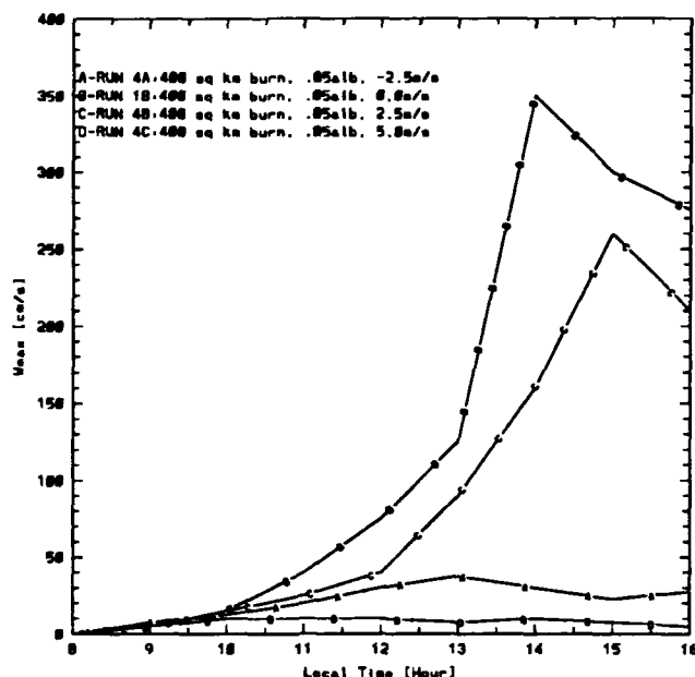
Figure 5.25: Diurnal variation of the vertical velocity field ( w ) for U_g = -2.5, 0.0, 2.5 , and 5.0 \text{ m s}^{-1} with burn area width/albedo = 400 \text{ sq km}/0.05 .
