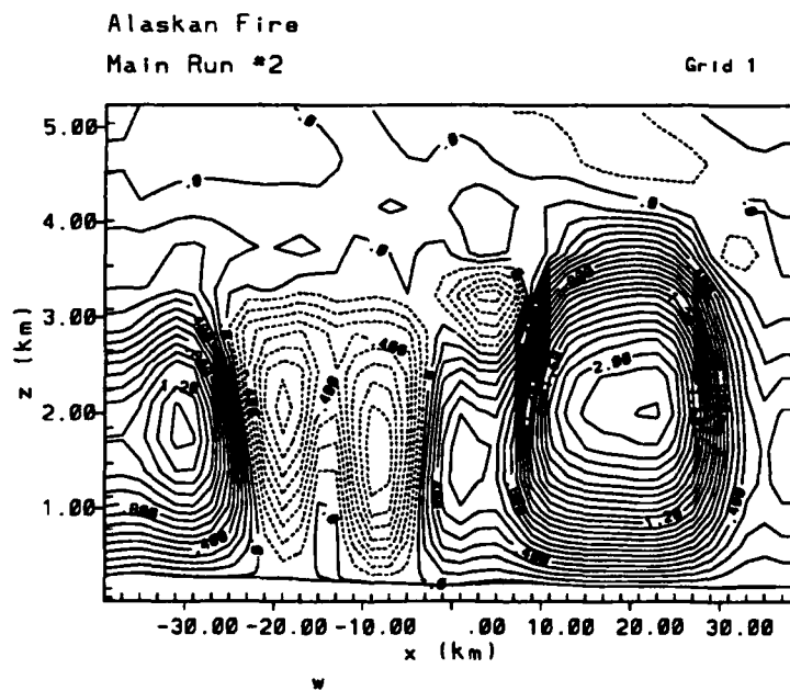
Figure 4.25: Vertical velocity field ( w ) in \text{cm s}^{-1} of Run 2 at 1400 LST, using a contour interval of 10 \text{ cm s}^{-1} .
