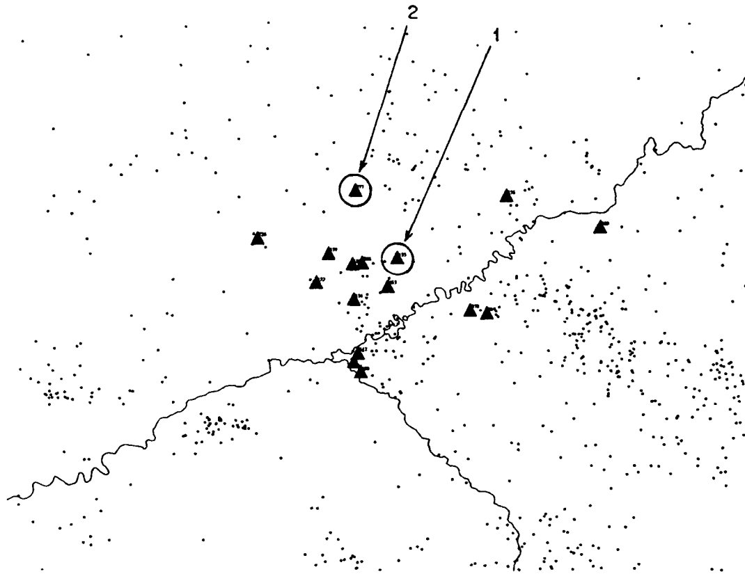
Figure 6.6: Lightning strike map of study area after Julian day 197.
