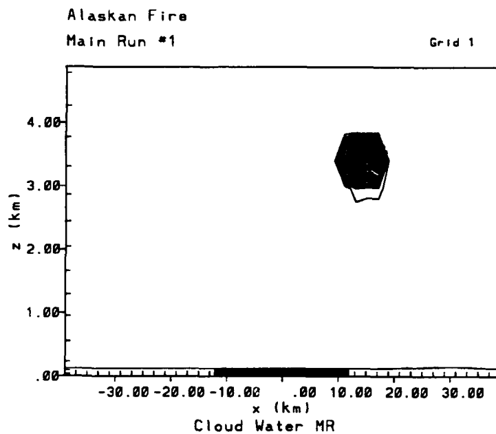
Figure 4.18: Cloud liquid water content ( \text{g kg}^{-1} ) of Run 1 at 1100 LST, using a contour interval of 0.02 \text{ g kg}^{-1} .
