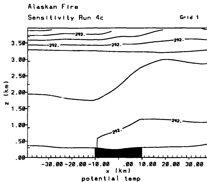
Figure 5.21: Potential temperature field ( \theta ) of Run 4c using U_g = 5.0 \text{ m s}^{-1} at 1400 LST, using a contour interval of 0.25^\circ\text{C} .
