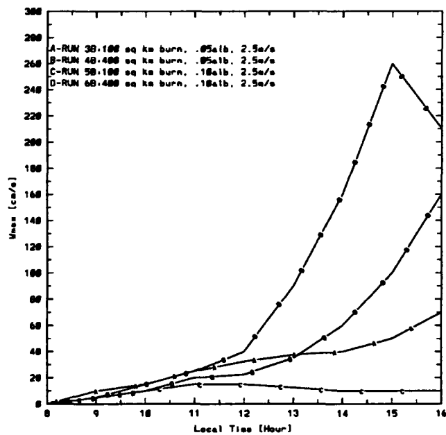
Figure 5.23: Diurnal variation of the vertical velocity field ( w ) for U_g = 2.5 \text{ m s}^{-1} geostrophic wind runs.
