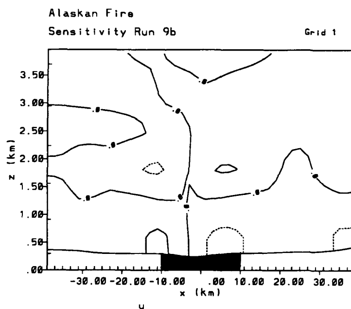
Figure 5.30: Horizontal velocity U component in \text{m s}^{-1} of Run 9b at 1500 LST, using a contour interval of 1 \text{ m s}^{-1} .
