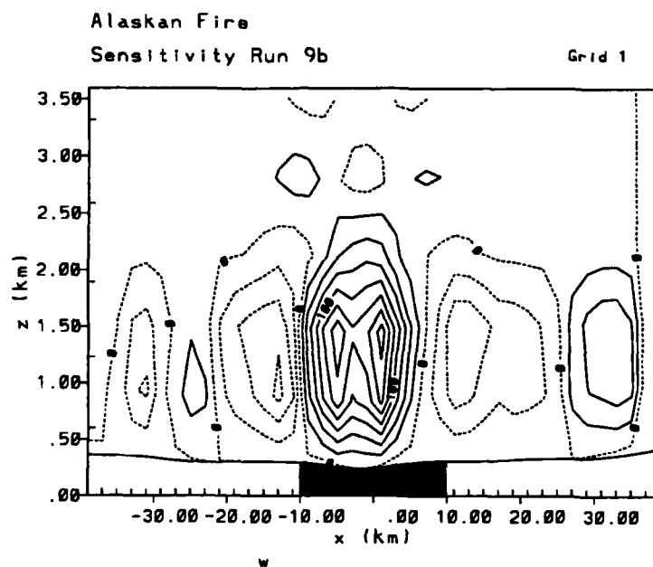
Figure 5.29: Vertical velocity field ( w ) in \text{cm s}^{-1} of Run 9b for a \frac{\partial \theta}{\partial z} = 9.0^\circ \text{C k}^{-1} at 1500 LST, using a contour interval of 2.5 \text{ cm s}^{-1} .
