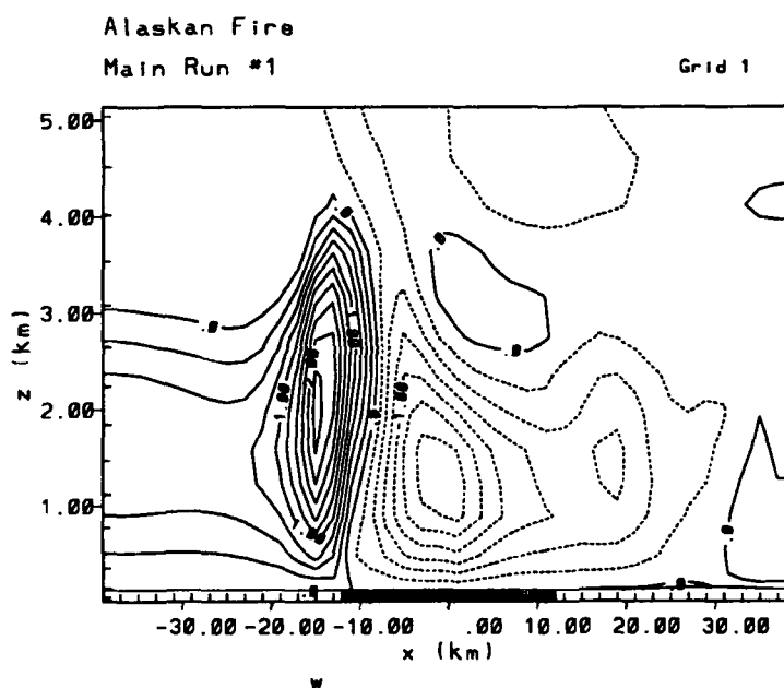
Figure 4.5: Vertical velocity field ( w ) in \text{cm s}^{-1} of Run 1 at 1600 LST, using a contour interval of 10 \text{ cm s}^{-1} .
