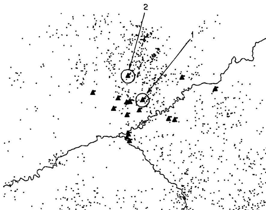
Figure 6.3: Lightning strike map of study area before Julian day 166.
