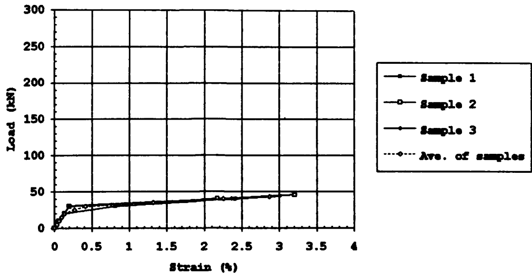
Figure A33. Load-Strain Data: V96/9.0 mm/SR24
