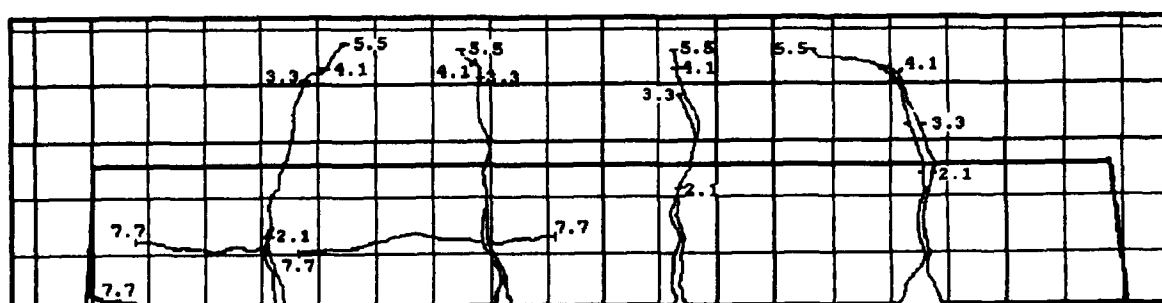
Figure B45. Crack Pattern Tracing: Test Beam #3 - K48/9.0 mm Hybrid Rod
