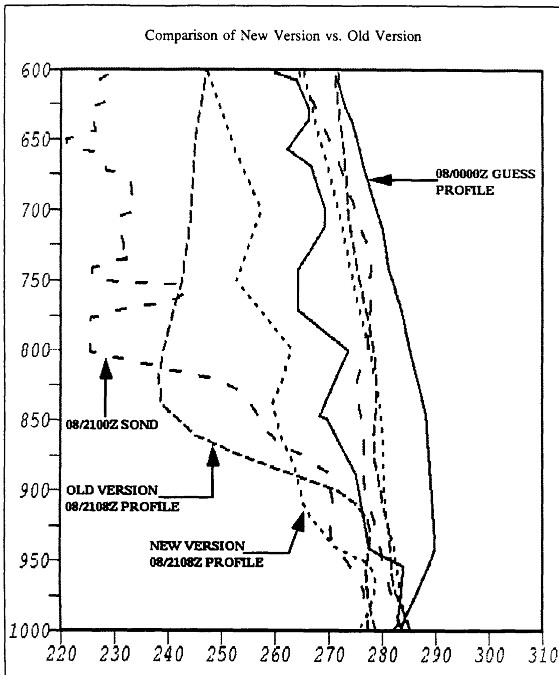
Figure 52: Comparison of new version 910508/2108 GMT profile (small dashed) with old version 910508/2108 GMT profile (medium dashed), 910508/2100 GMT rawinsonde profile (large dashed) and the 910508/0000 GMT guess profile (solid).
