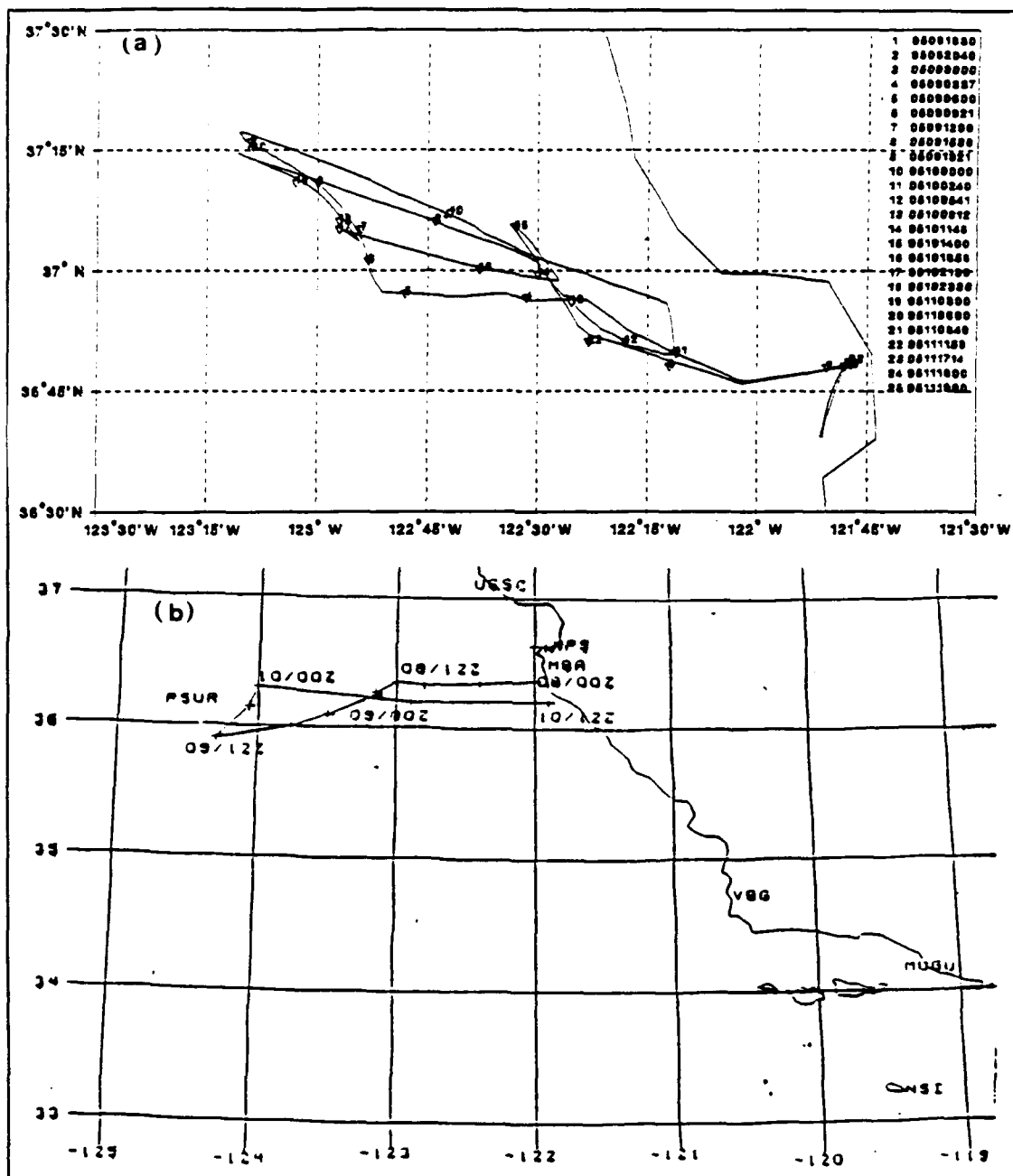
Figure 7: Plot of the ship paths for each of the research cruises. The 1992 cruise is depicted in (a) and the 1991 cruise is in (b).
