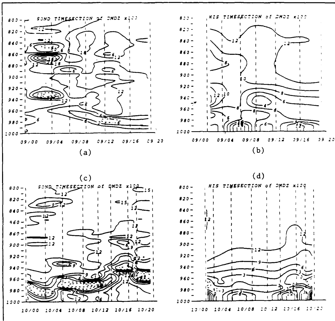
Figure 53: Timesections of \delta M / \delta Z on 9 and 10 May 1992 for the rawinsonde, (a) and (c), and the GB-HIS, (b) and (d), data. \delta M / \delta Z values are scaled by a factor of 100. Dashed lines indicate negatives values.
