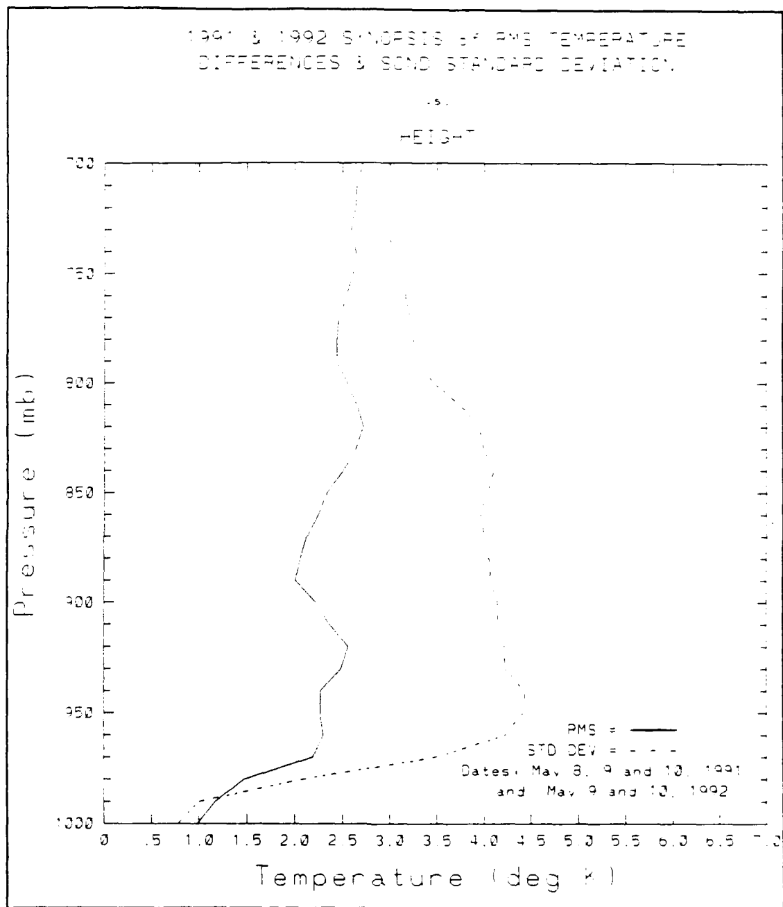
Figure 49: Root mean squared temperature differences are compared to atmospheric standard deviation for the 1991 and 1992 cruises combined. Skill is noted when rms is less than std dev. (Old Version)
