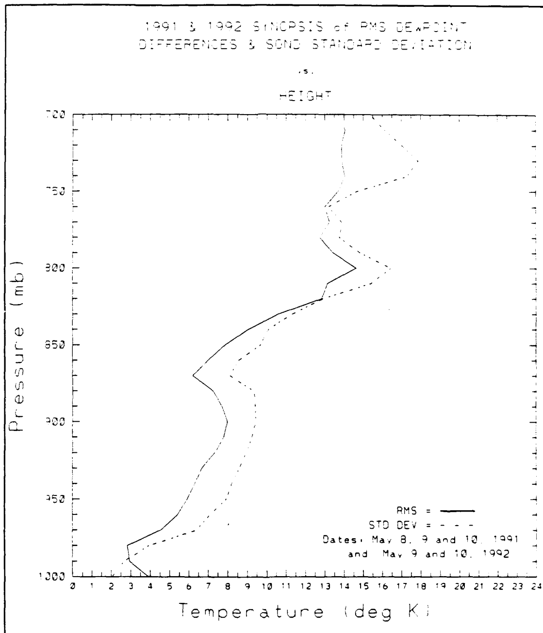
Figure 46: Root mean squared dewpoint differences are compared to atmospheric standard deviation for the 1991 and 1992 cruises combined. Skill is noted when rms is less than std dev. (New Version)
