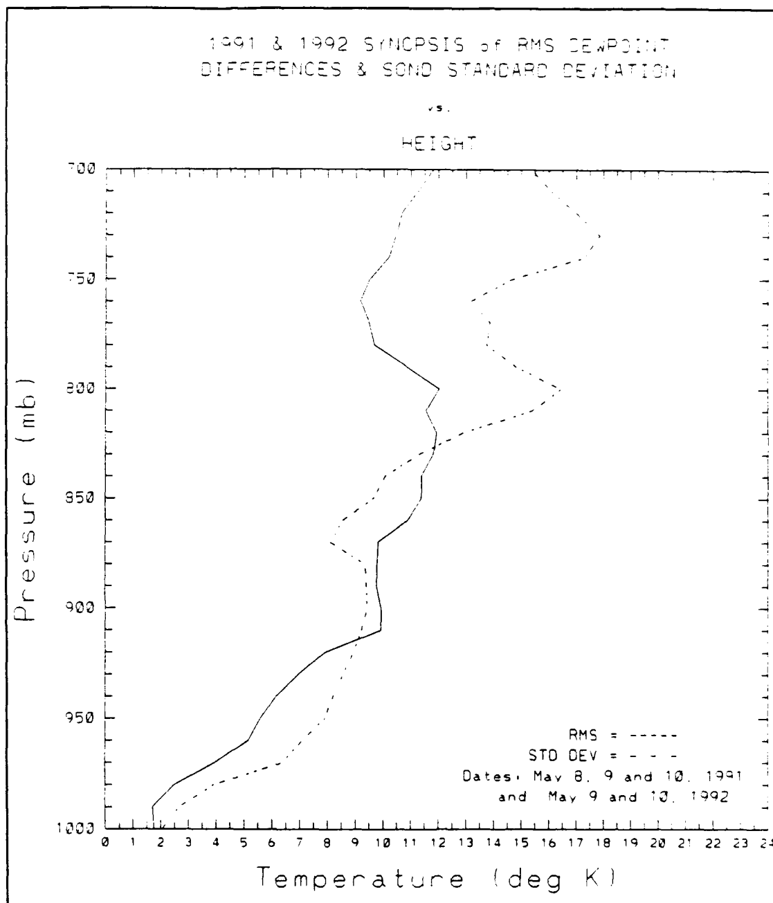
Figure 47: Root mean squared dewpoint differences are compared to atmospheric standard deviation for the 1991 and 1992 cruises combined. Skill is noted when rms is less than std dev. (Old Version)
