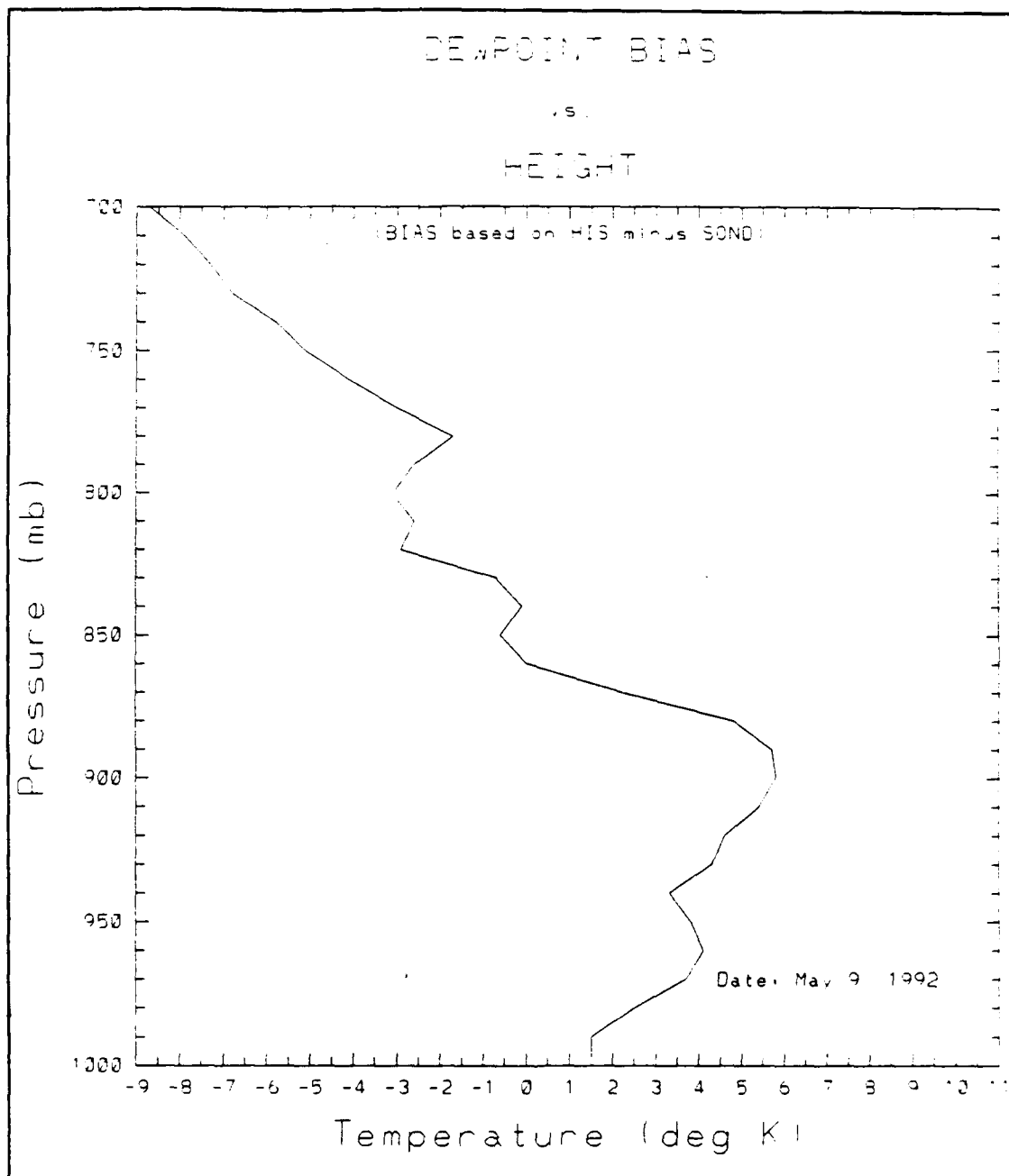
Figure 37: Dewpoint bias profile based on the value of the HIS minus the value of the rawinsonde at the same level. A positive bias indicates an overestimation and a negative bias an underestimation of dewpoint.
