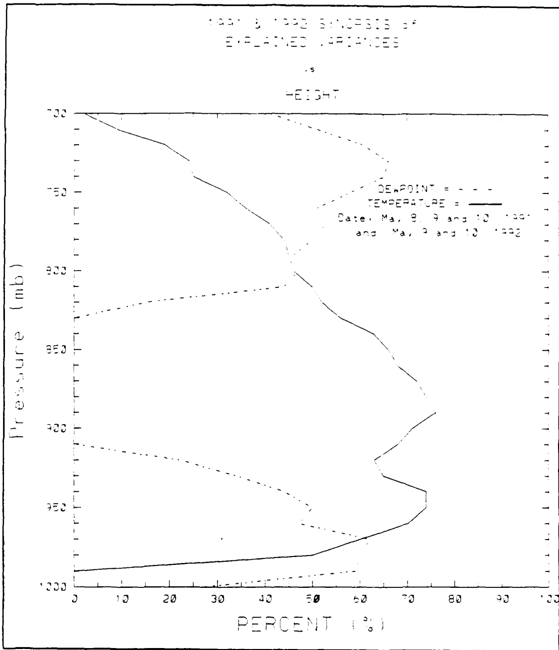
Figure 51: The quantity of atmospheric variance of dewpoint and temperature profiles explained by the HIS. Variance is based on the 0000 GMT rawinsonde profile for each of the days of each cruise. (Old Version)
