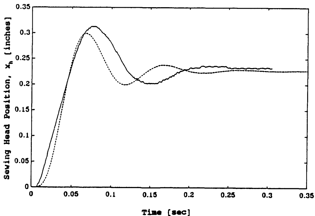
Figure 3.21. X axis motor shaft and sewing head position step response, actual system and model.
