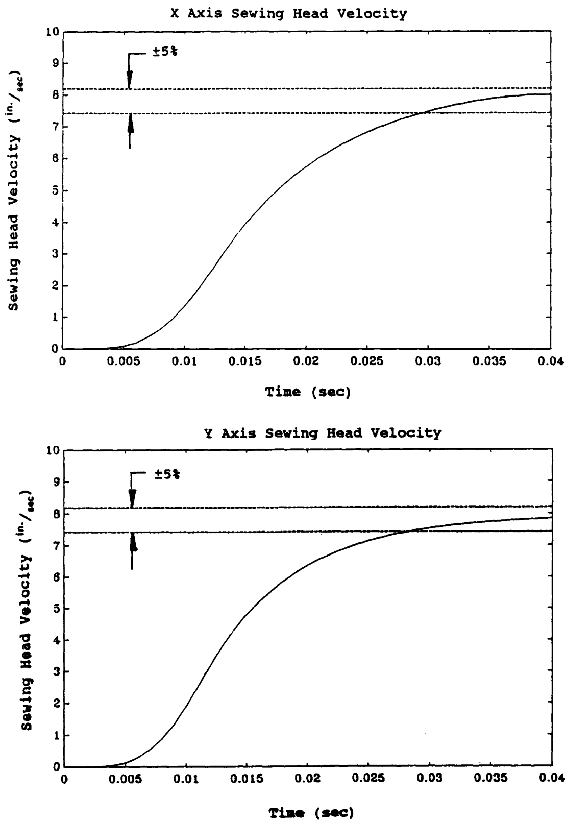
Figure 4.21. The nonlinear model velocity response simulation.
