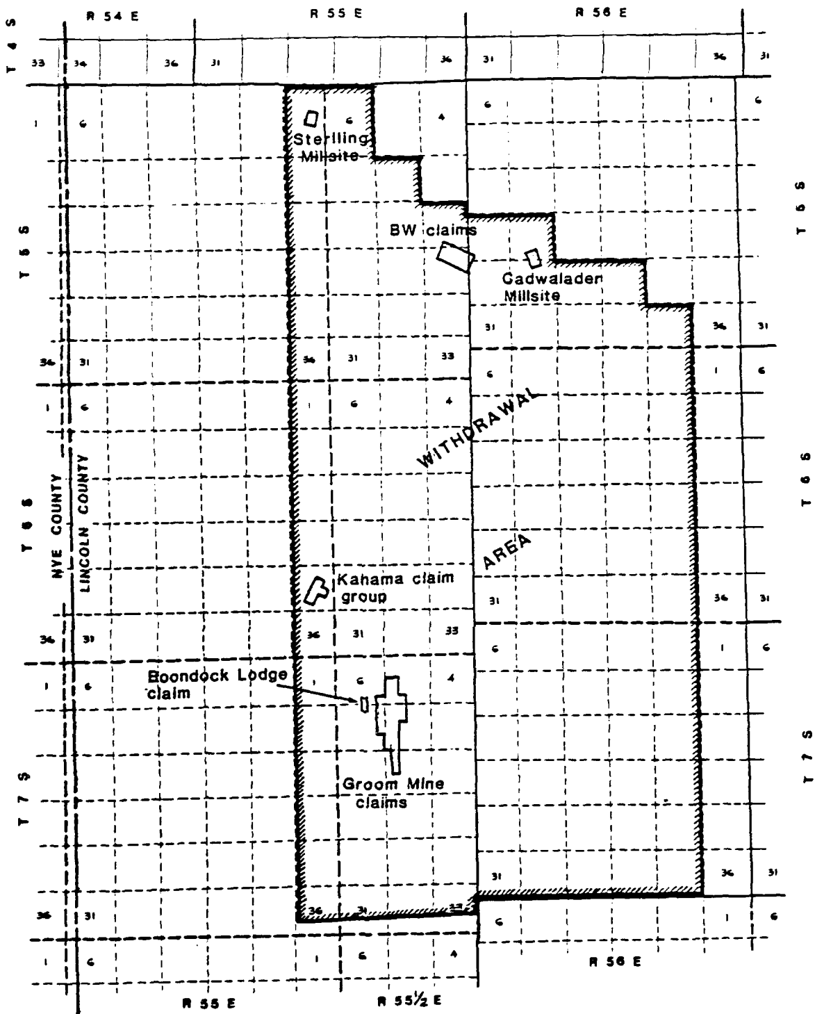
FIGURE 3.7 (Revised) Patented and Unpatented Mining Claims Location Map Groom Mountain Range Withdrawal
