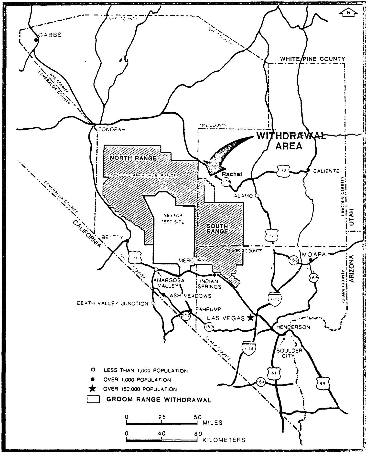
FIGURE 1.1 (Revised) Generalized Location Map - Groom Mountain Range Withdrawal
