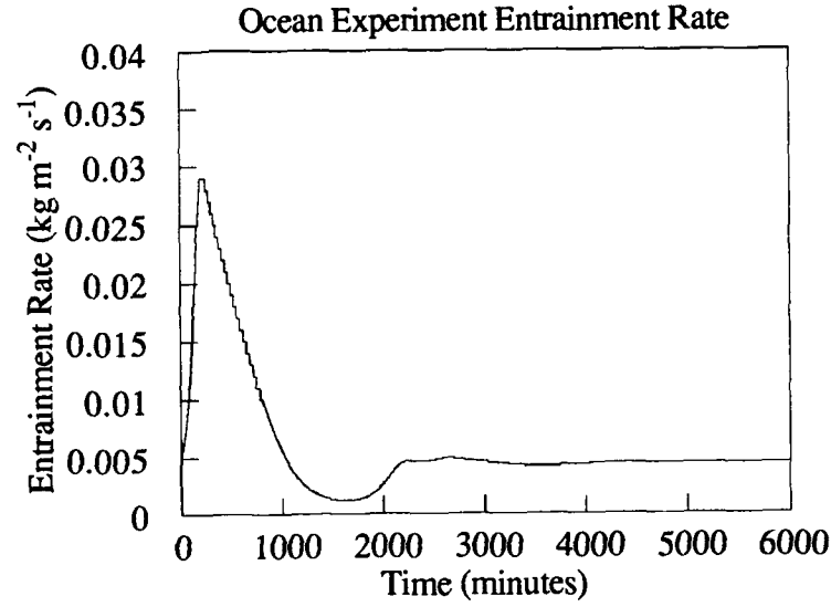
Figure 5.b.7: E for Ocean Experiment.
