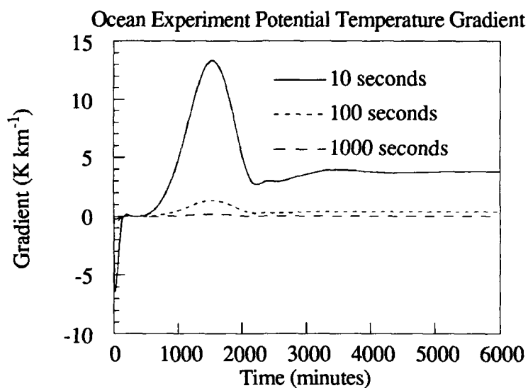
Figure 7.f.4: \frac{\partial \theta}{\partial z} with \hat{\tau} = 10, 100, and 1000 Seconds for Ocean Experiment.
