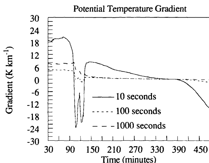
Figure 7.b.4: \frac{\partial \bar{\theta}}{\partial z} with \hat{\tau} = 10, 100, \text{ and } 1000 Seconds for Wangara Day 33 0930-1600L.
