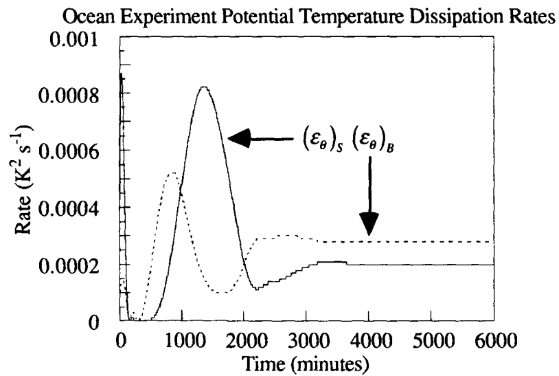
Figure 7.f.2: (\epsilon_\theta)_S and (\epsilon_\theta)_B for Ocean Experiment.
