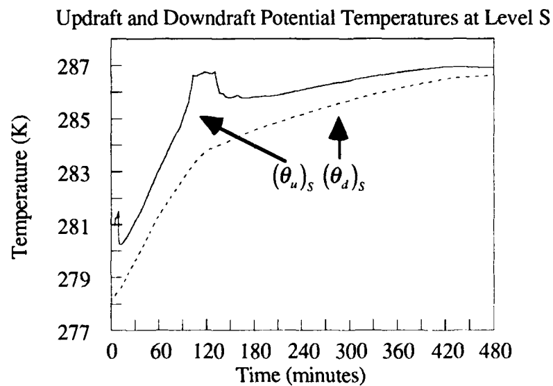
Figure 7.a.4: (\theta_u)_s and (\theta_d)_s for Wangara Day 33 0900-1600L.
