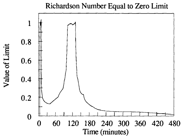
Figure 7.d.2: Ri=0 Limit for Wangara Day 33 0900-1600L.
