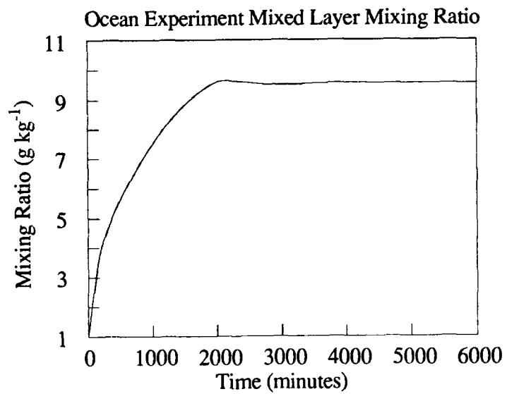
Figure 5.b.3: Predicted q_m Over Ocean.
