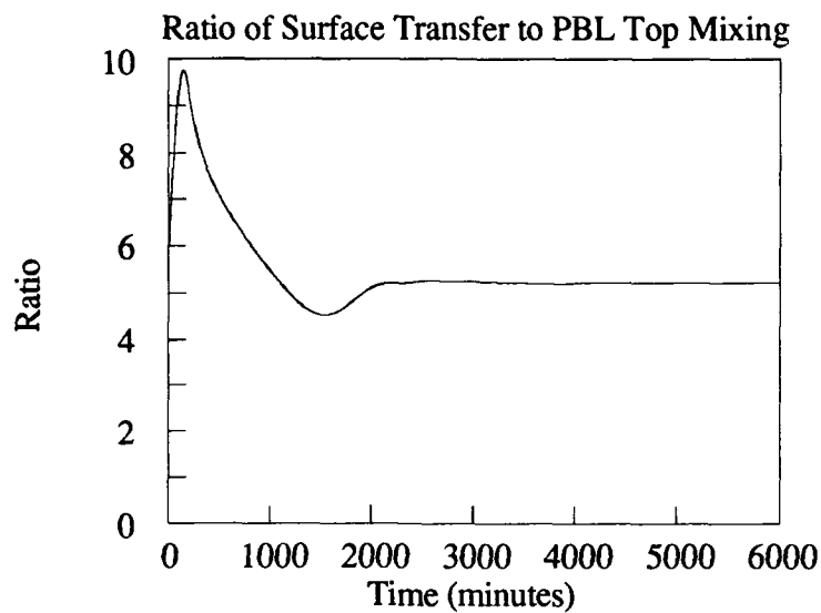
Figure 5.b.6: A for Ocean Experiment.
