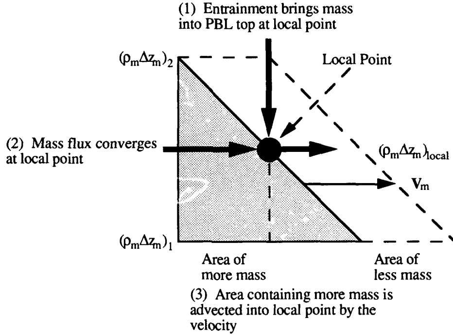
Figure 2.a.(2).1: Processes Which Cause Local Change in Mass.
