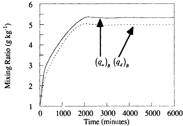
Ocean Experiment Up/Down Mixing Ratios at Level B
