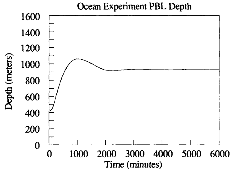
Figure 5.b.1: Predicted \Delta z_m Over Ocean.
