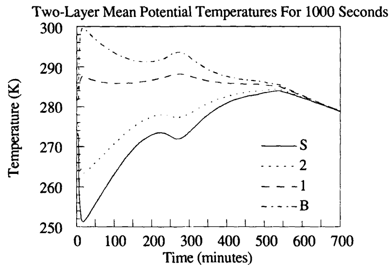
Figure 9.b.6: Mean Potential Temperatures Using \hat{\tau} = 1000 Seconds.
