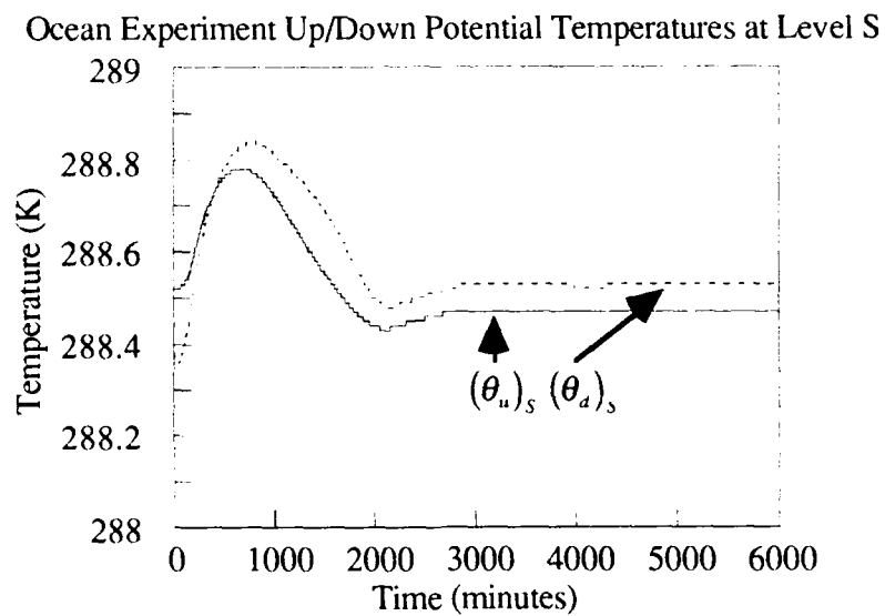
Figure 7.e.4: (\theta_u)_s and (\theta_d)_s for Ocean Experiment.
