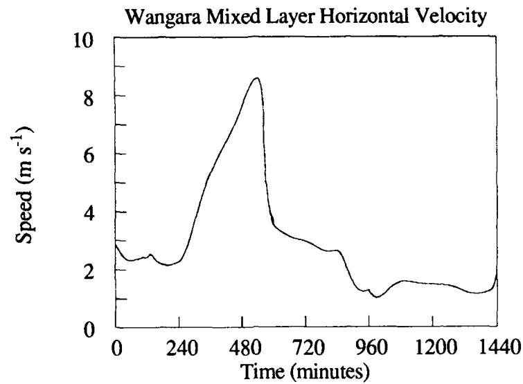
Figure 5.a.(1).5: Predicted Diurnal |v_m| for Wangara Day 33.
