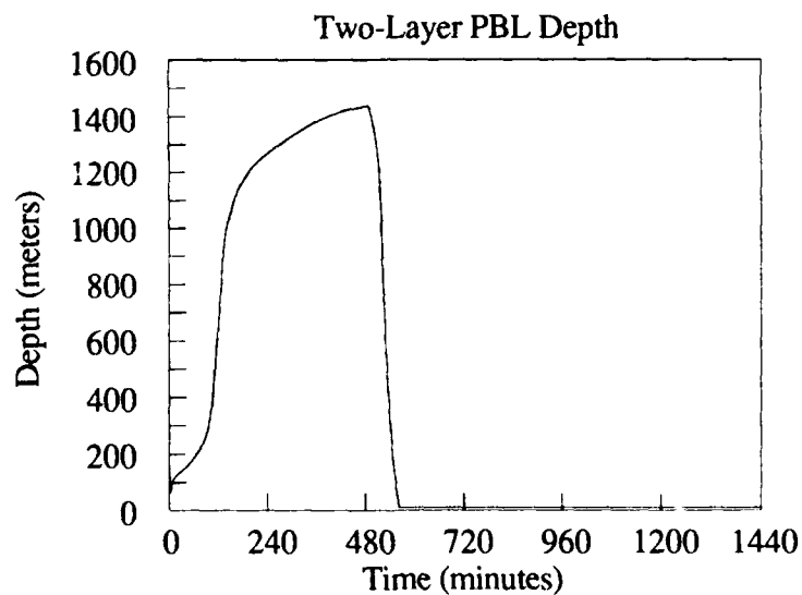
Figure 9.a.1: Two-Layer \Delta z_m .
