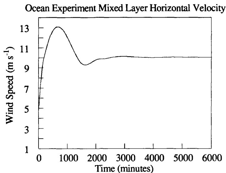
Figure 5.b.4: Predicted |v_m| Over Ocean.
