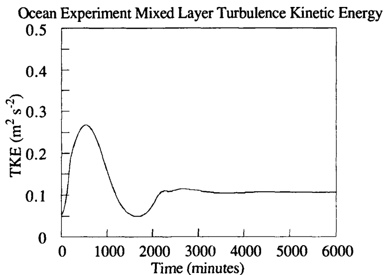
Figure 5.b.5: Predicted e_m Over Ocean.
