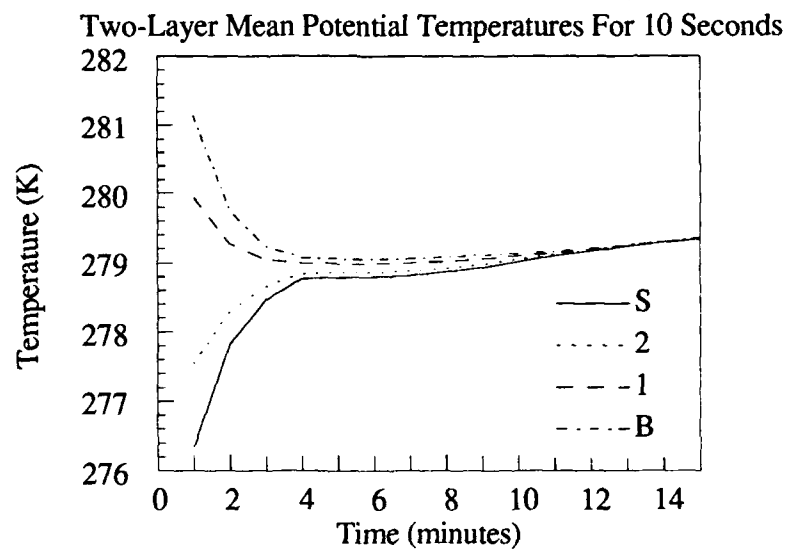
Figure 9.b.4: Mean Potential Temperatures Using \hat{\tau} = 10 Seconds.
