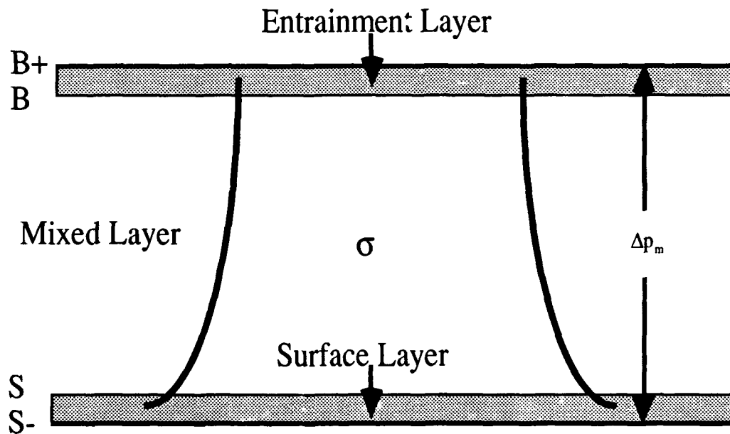
Figure 1.b.1: Domain of Bulk Boundary Layer Model.
