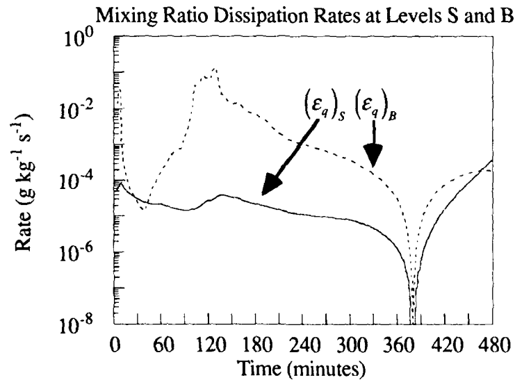
Figure 7.b.3: (\epsilon_q)_S and (\epsilon_q)_B for Wangara Day 33 0900-1600L.
