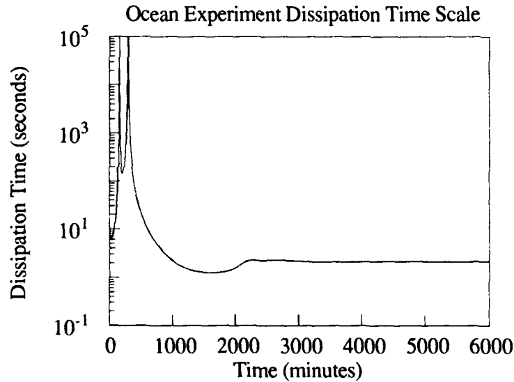
Figure 7.f.1: \tau_{dis} for Ocean Experiment.
