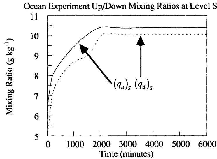
Figure 7.e.5: (q_u)_s and (q_d)_s for Ocean Experiment.
