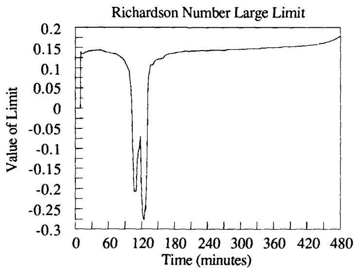
Figure 7.d.3: Ri \gg 1 Limit for Wangara Day 33 0900-1600L.
