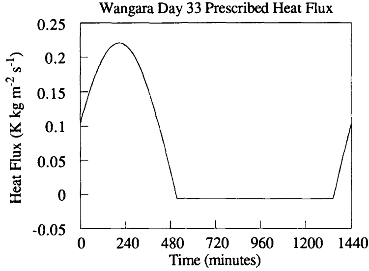
Figure 3.c.1: Prescribed Wangara Day 33 Surface Heat Flux From André et al. (1978)
