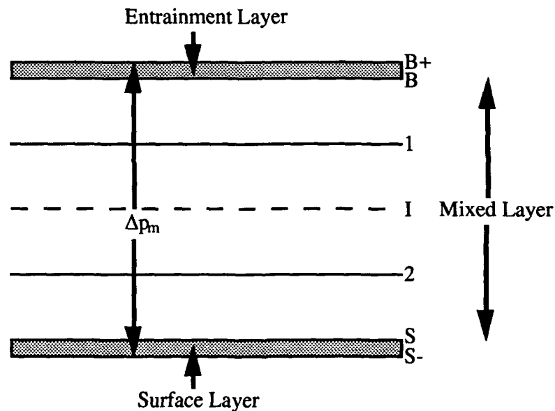
Figure 8.1: Illustration of 2-Layer Model.
