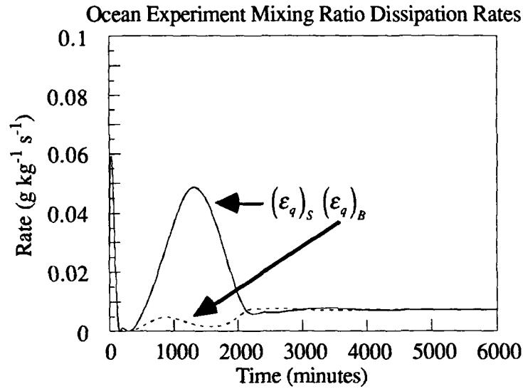
Figure 7.f.3: (\epsilon_q)_s and (\epsilon_q)_B for Ocean Experiment.
