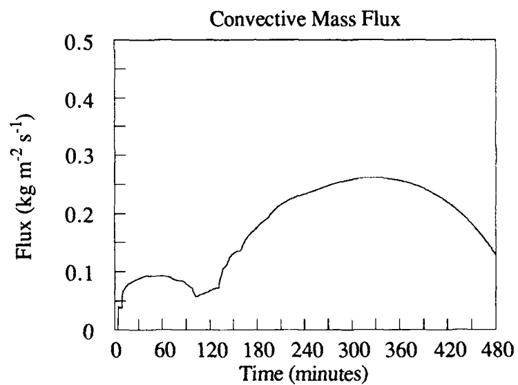
Figure 7.a.3: M_C for Wangara Day 33 0900-1600L.
