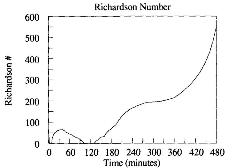
Figure 7.d.1: Ri for Wangara Day 33 0900-1600L.
