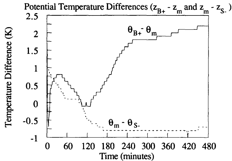
Figure 5.a.(1).2: Diurnal \theta_m - \theta_{S-} and \theta_{B+} - \theta_m for Wangara Day 33.
