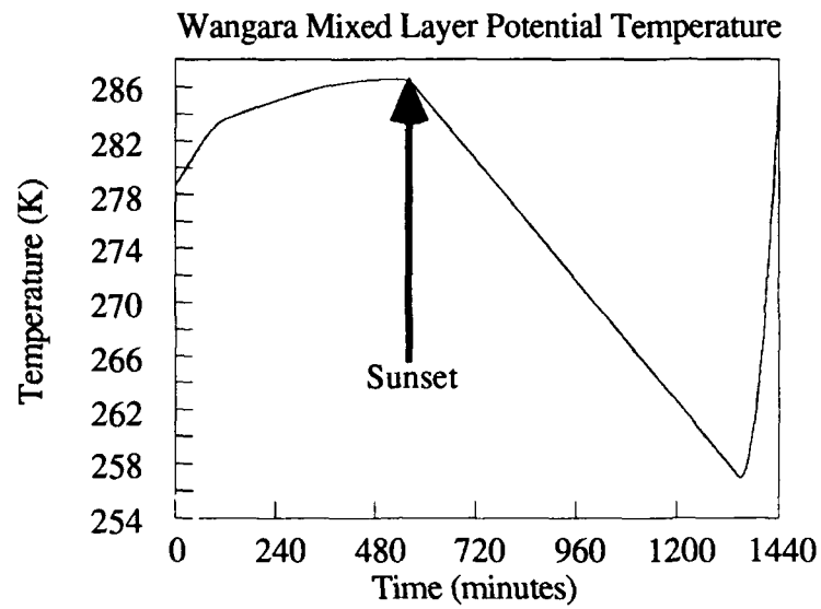
Figure 5.a.(1).3: Predicted Diurnal \theta_m for Wangara Day 33.
