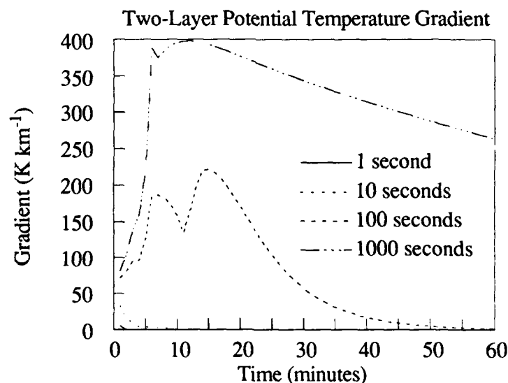
Figure 9.b.1: \frac{\partial \bar{\theta}}{\partial z} with \hat{\tau} = 1, 10, 100, \text{ and } 1000 \text{ Seconds} for Two-Layer Model.
