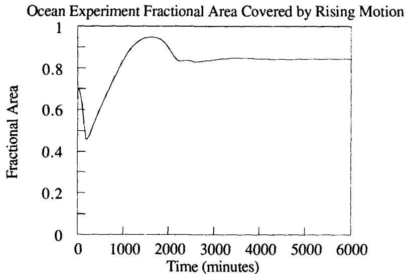
Figure 7.e.1: \sigma for Ocean Experiment.
