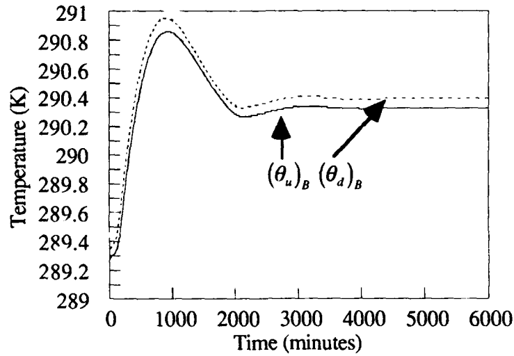
Ocean Experiment Up/Down Potential Temperatures at Level B
