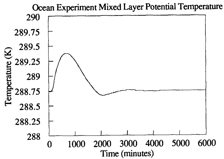
Figure 5.b.2: Predicted \theta_m Over Ocean.
