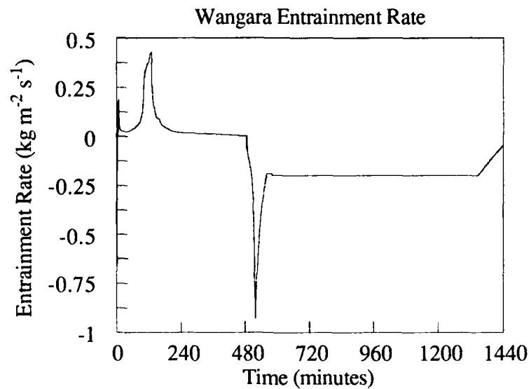
Figure 5.a.(1).9: Predicted Diurnal E Wangara Day 33.
