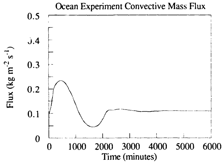
Figure 7.e.3: M_C for Ocean Experiment.
