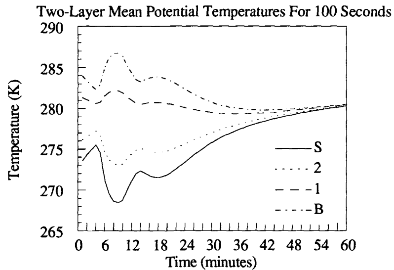
Figure 9.b.5: Mean Potential Temperatures Using \hat{\tau} = 100 Seconds.
