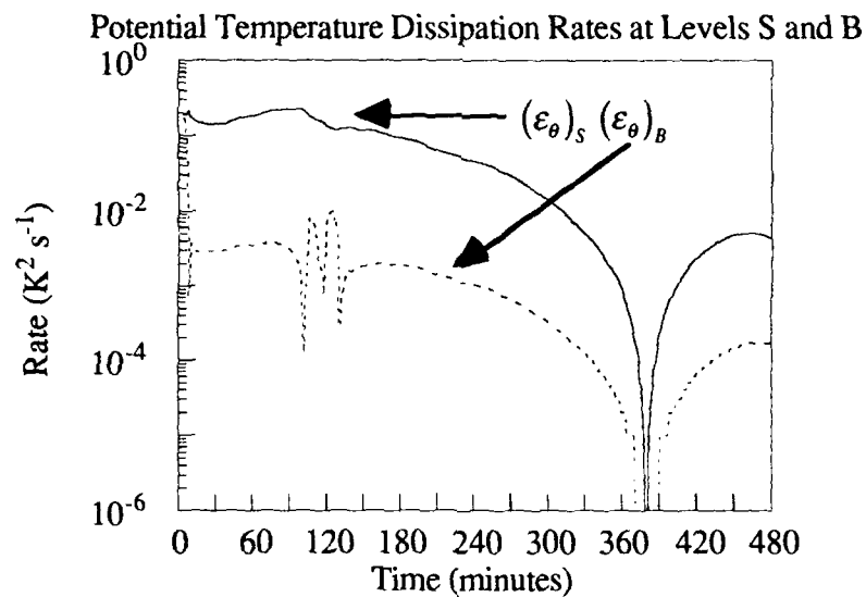
Figure 7.b.2: (\epsilon_\theta)_S and (\epsilon_\theta)_B for Wangara Day 33 0900-1600L.
