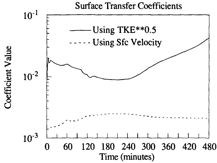
Figure 7.c.1: C_T and C_{T'} for Wangara Day 33 0900-1600L.
