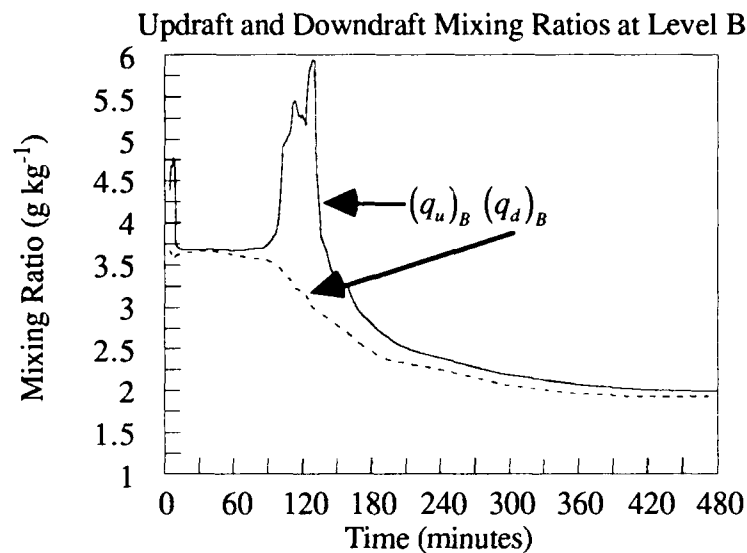
Figure 7.a.7: (q_u)_B and (q_d)_B for Wangara Day 33 0900-1600L.
