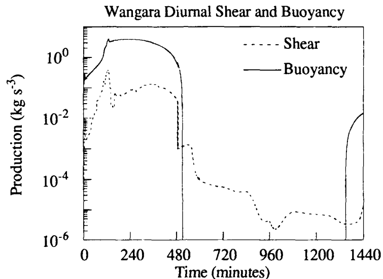
Figure 5.a.(1).8: Diurnal B and S Wangara Day 33.
