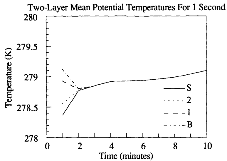
Figure 9.b.3: Mean Potential Temperatures Using \hat{\tau} = 1 Second.
