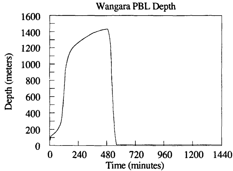
Figure 5.a.(1).1: Predicted Diurnal \Delta z_m for Wangara Day 33.
