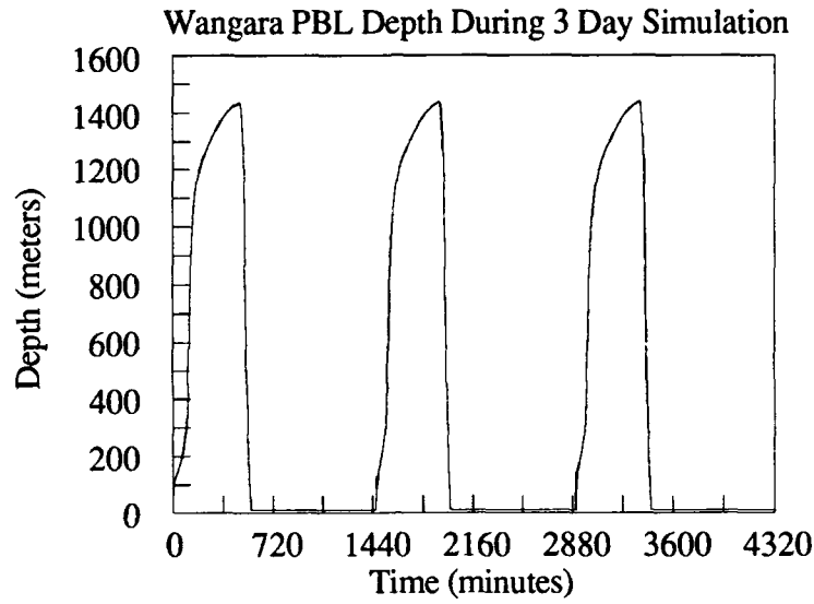
Figure 5.a.(2).1: Predicted 3 Day \Delta z_m Reusing Wangara Day 33 Data Each Day.
