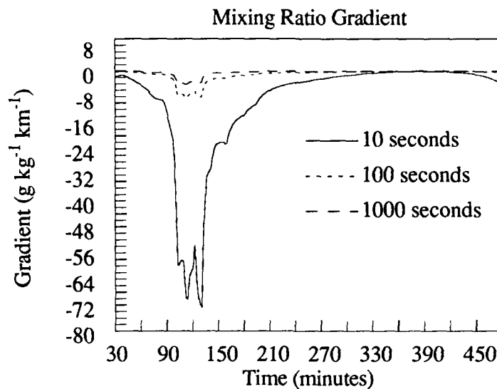
Figure 7.b.5 \frac{\partial \bar{q}}{\partial z} with \hat{\tau} = 10, 100, \text{ and } 1000 \text{ Seconds} for Wangara Day 33 0930-1600L.
