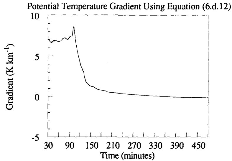
Figure 7.b.6: \frac{\partial \bar{\theta}}{\partial z} Using (6.d.12) for Wangara Day 33 0930-1600L.
