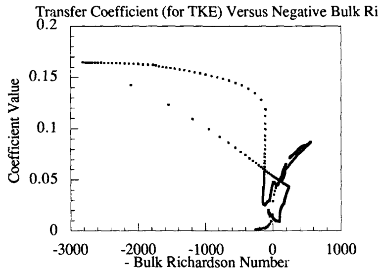
Figure 7.c.2: Scatter Plot of C_{T'} Versus -Ri_{Bulk} for Wangara Day 33 0900-1600L.
