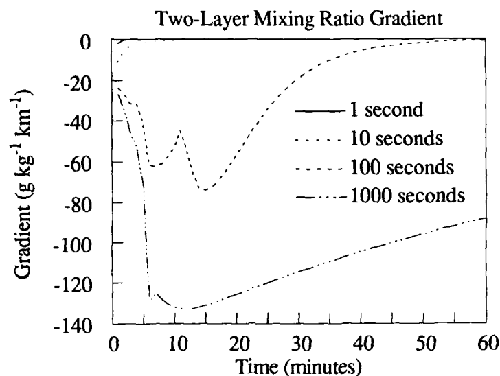
Figure 9.b.2: \frac{\partial \bar{q}}{\partial z} with \hat{\tau} = 1, 10, 100, and 1000 Seconds for Two-Layer Model.
