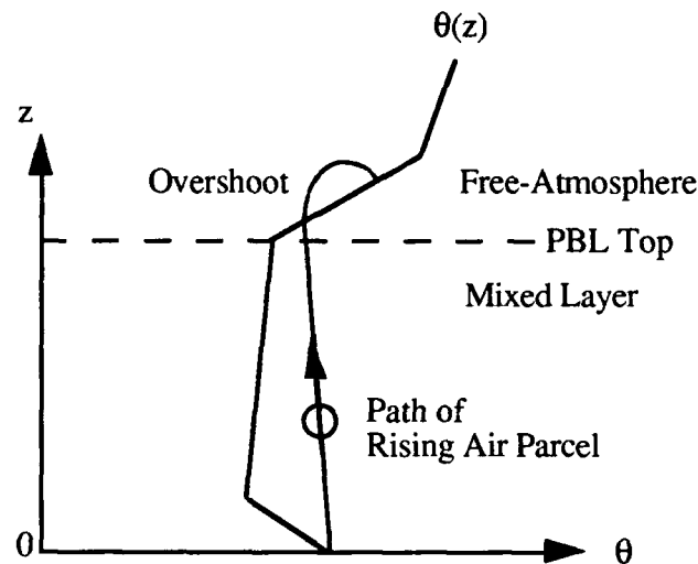
Figure 5.a.(1).7: Illustration of the Process of Penetrative Convection (Stull, 1991).
