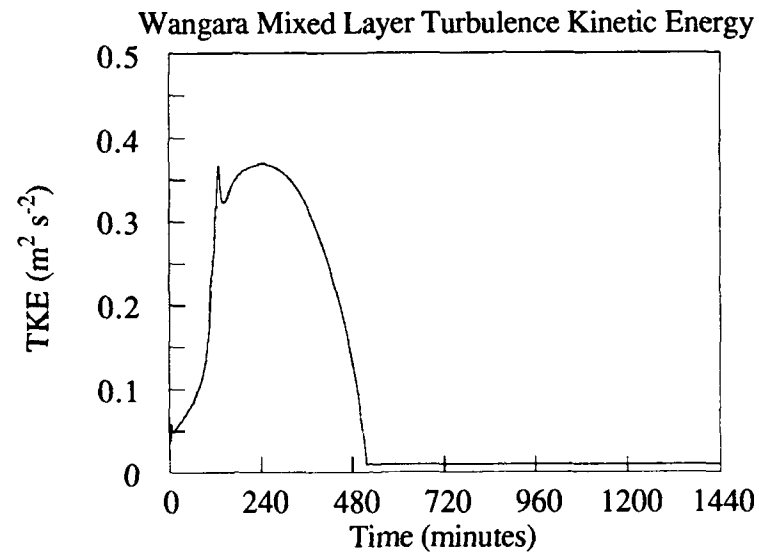
Figure 5.a.(1).6: Predicted Diurnal e_m for Wangara Day 33.
