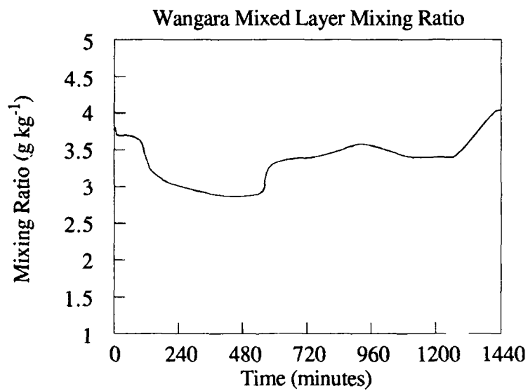
Figure 5.a.(1).4: Predicted Diurnal q_m for Wangara Day 33.
