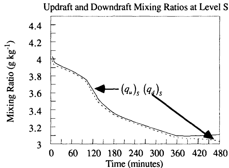
Figure 7.a.5: (q_u)_s and (q_d)_s for Wangara Day 33 0900-1600L.
