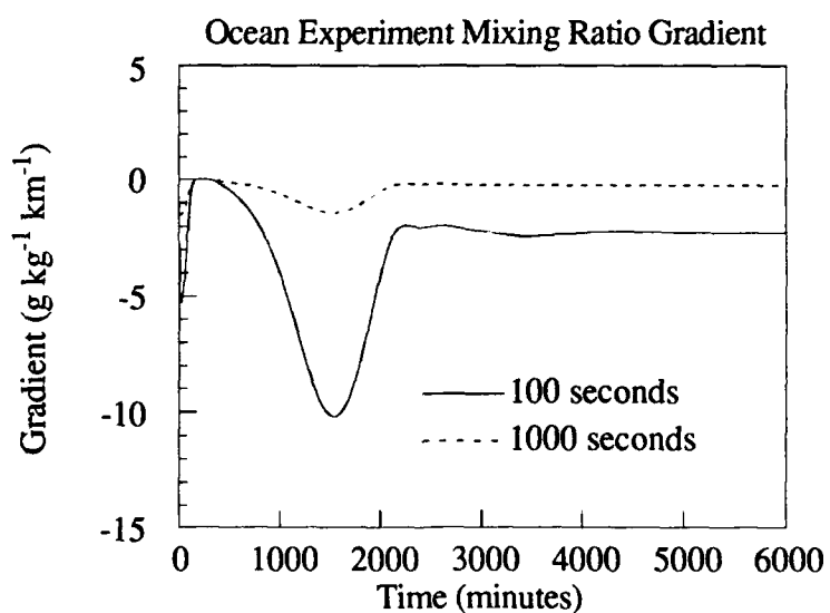
Figure 7.f.5: \frac{\partial q}{\partial z} with \hat{\tau} = 10, 100, and 1000 Seconds for Ocean Experiment.
