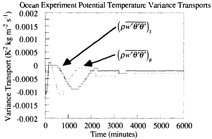
Figure 7.e.2: (\overline{\rho w' \theta' \theta'})_s and (\overline{\rho w' \theta' \theta'})_B for Ocean Experiment.
