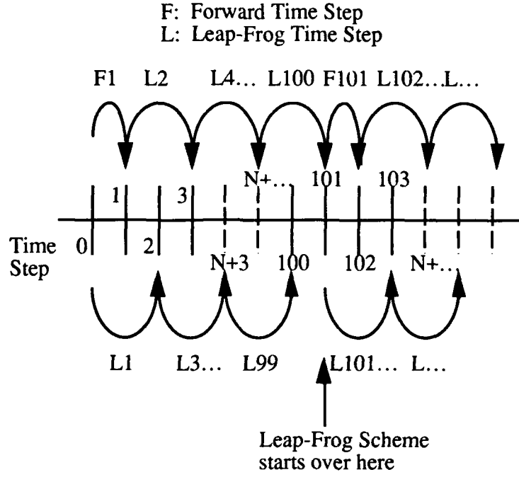
Figure 3.b.1: Conservation of Momentum Time Scheme Flow Diagram
