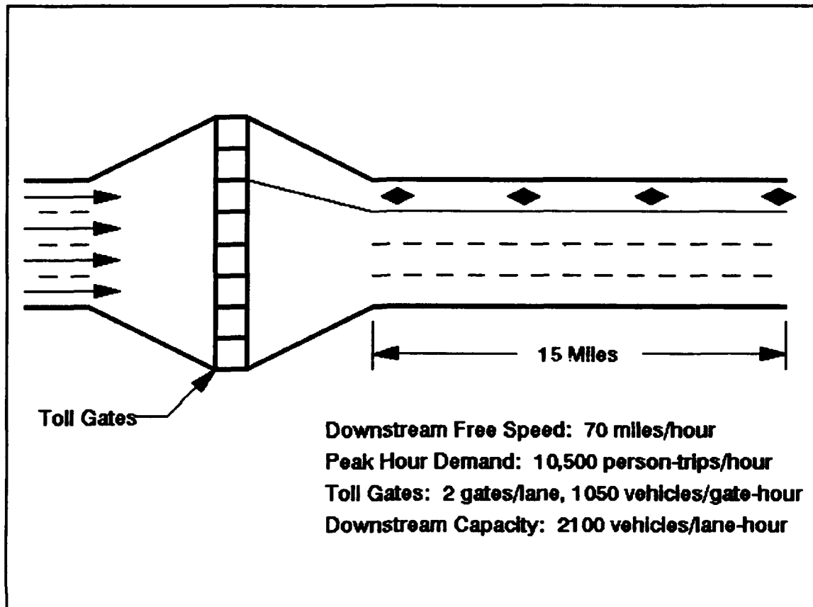
Figure 1 - Highway Facility
