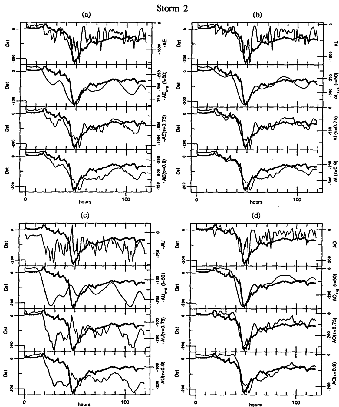
Fig. A.2. Plots for storm 2. Dst (bold) is plotted versus AE , AE_{avg} , AE(\tau=0.75) , and AE(\tau=0.9) (a). The same is done for AL (b), AU (c), and AO (d).
