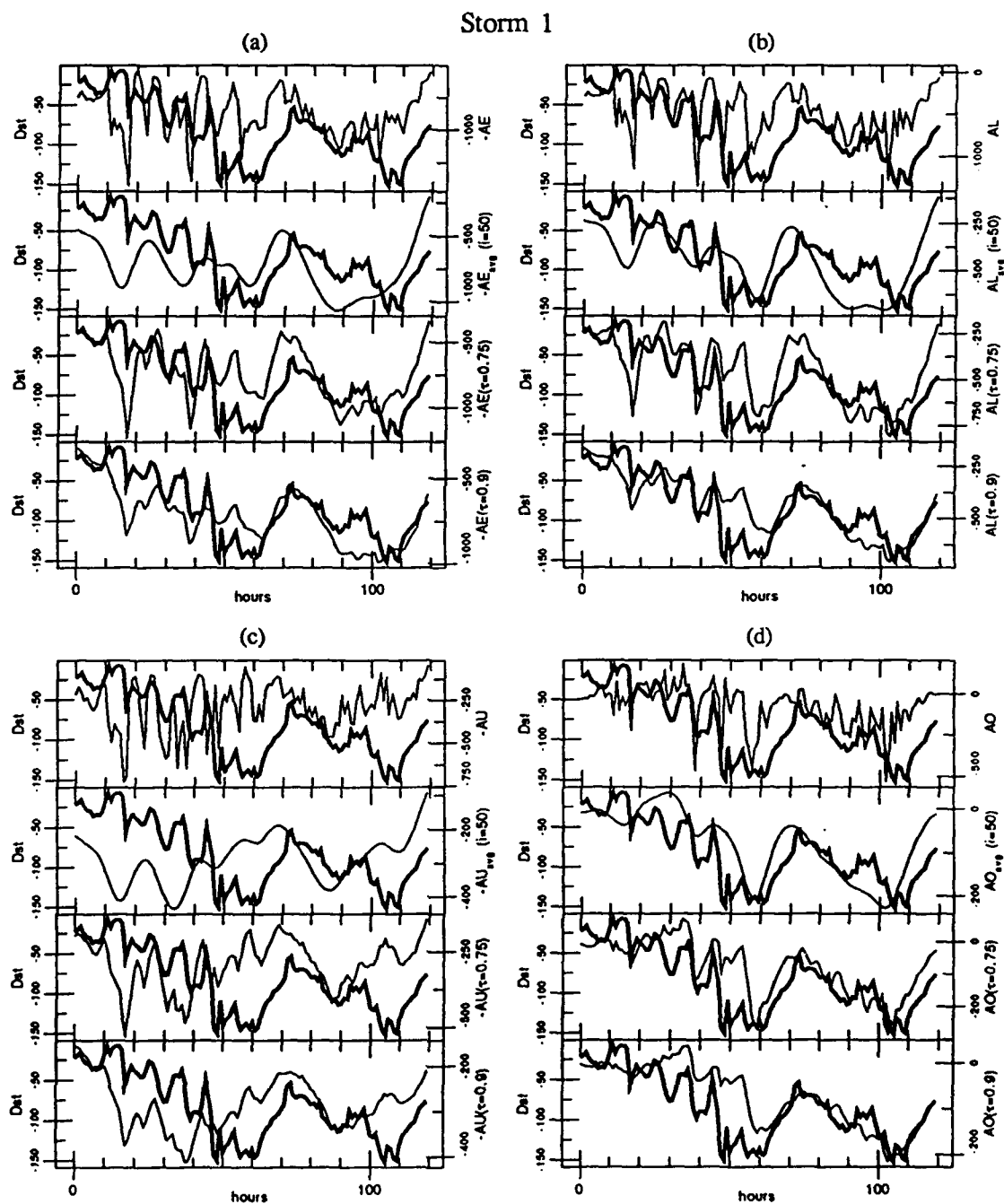
Fig. A.1. Plots for storm 1. Dst (bold) is plotted versus AE , AE_{avg} , AE(\tau=0.75) , and AE(\tau=0.9) (a). The same is done for AL (b), AU (c), and AO (d).
