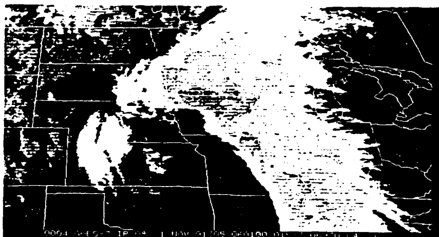
Fig. 21 Satellite imagery using a winter enhancement curve for 0600 UTC 1 November 1991.
