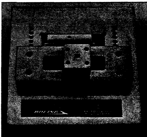
b) Traveling Transition to Measure RF Level and Phase Delivered by the Feed Network to Each of the 93 Honeycomb Waveguides
