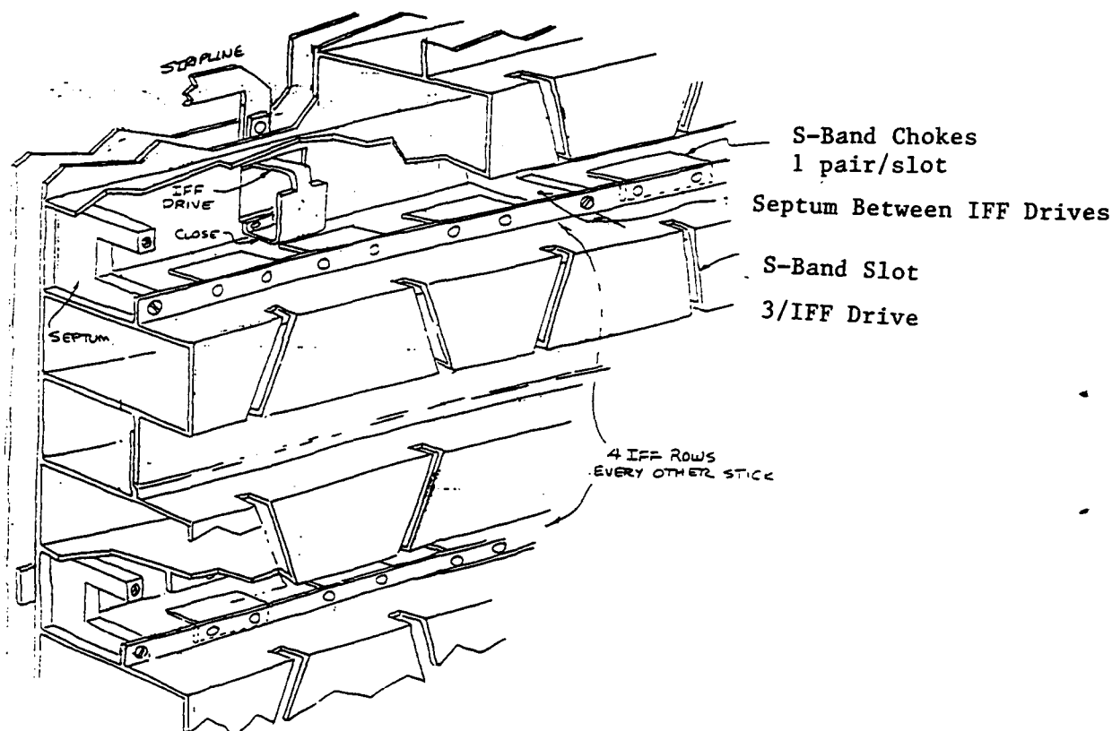
Figure 2. Integral IFF Antenna
