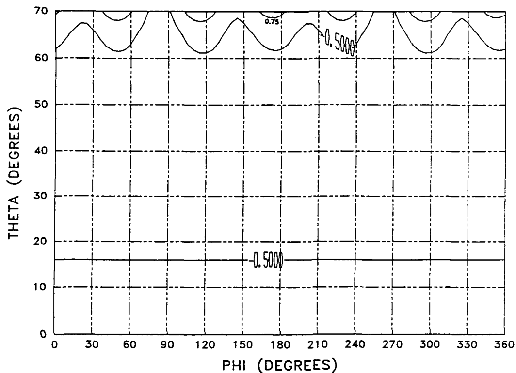
Figure 15. Reflection Loss dB, 2 Layer WAIM, \epsilon_r = 3.37 at 20.2 GHz RHCP
