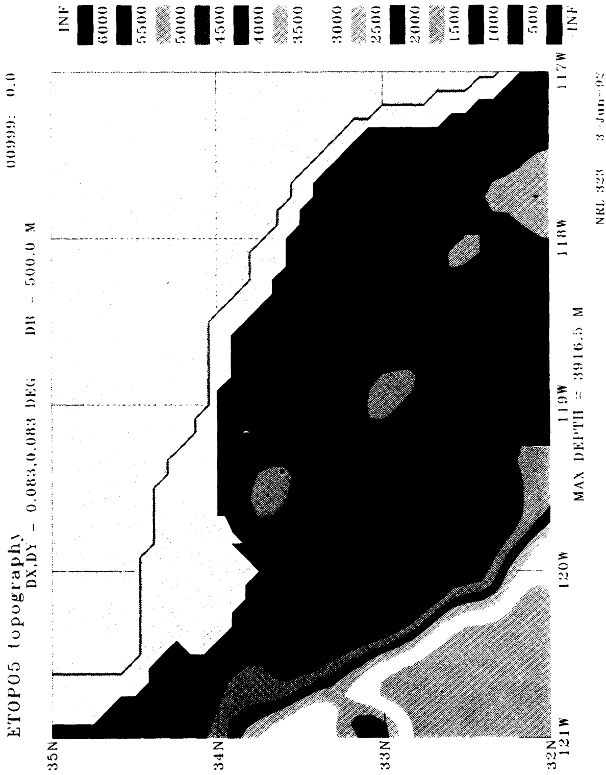
Figure 14: Plot of the Channel Islands west of Los Angeles, California from the 1/12° ETOPO5 topography.
