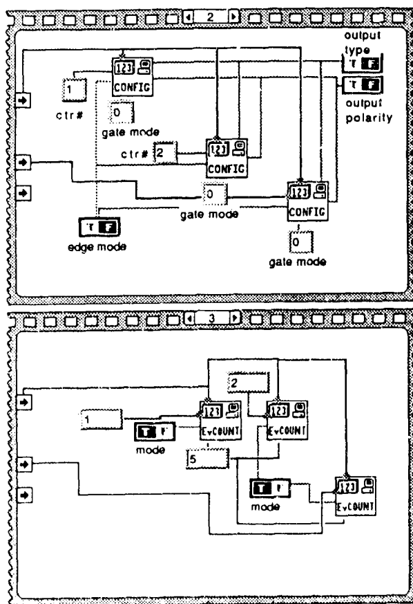
Figure A-3. Frames 2 and 3 within Counter routine: counters are configured and counting is started.
