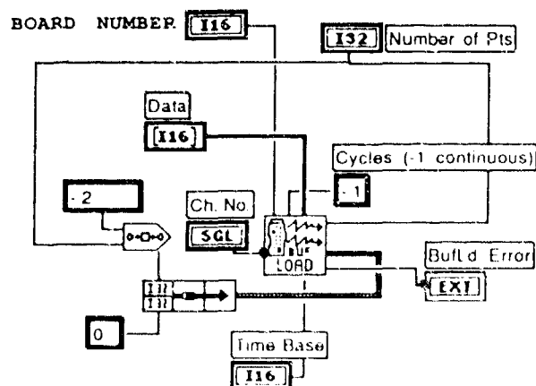
Figure C-1. Connector Panel, Front Panel and Block Diagram for sub-VI, Setup Dble Buffering.
