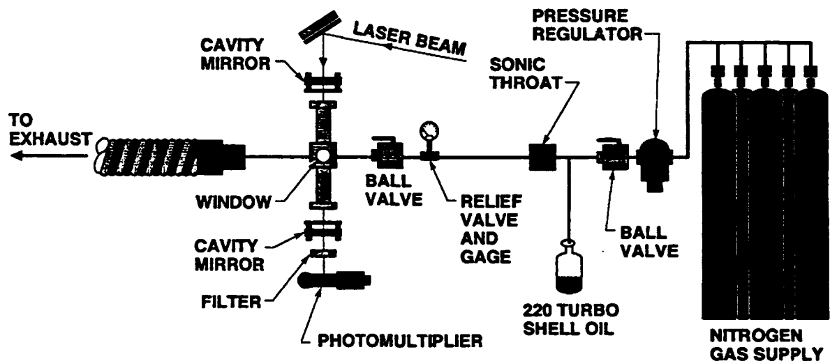
Figure 11. Schematic of test apparatus with no filters to demonstrate sensitivity of laser diagnostic technique (Runs 9-14).
