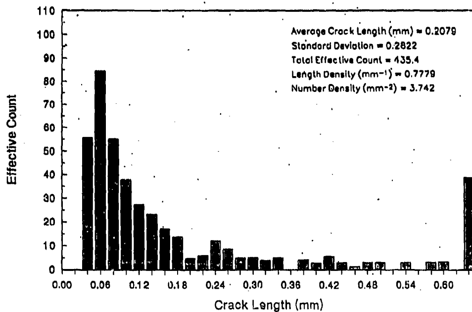
Crack Length Distribution Transverse Bundle Cracks - Specimen 1652-16 - X
