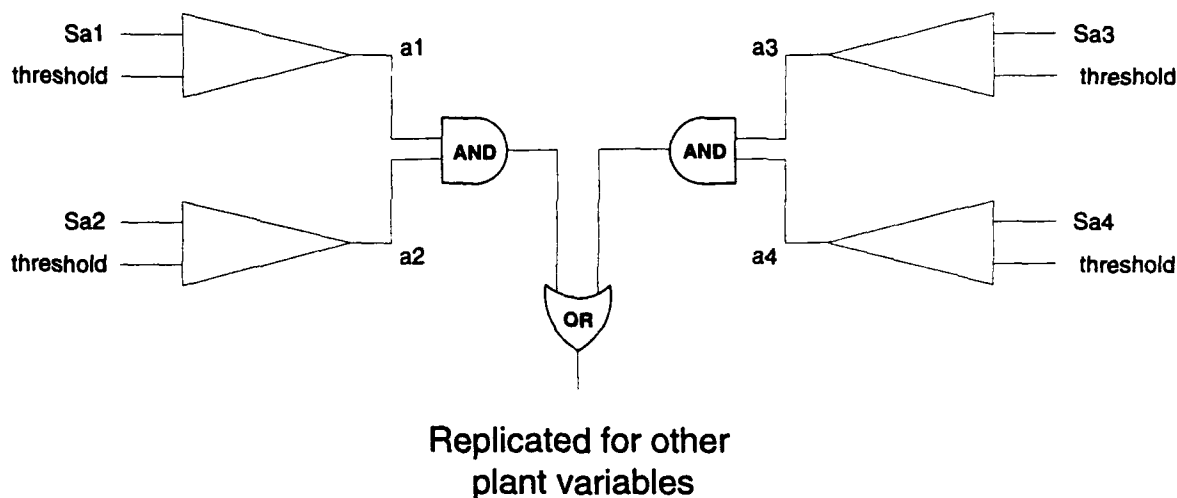
Figure B.1: Analog Implementation
