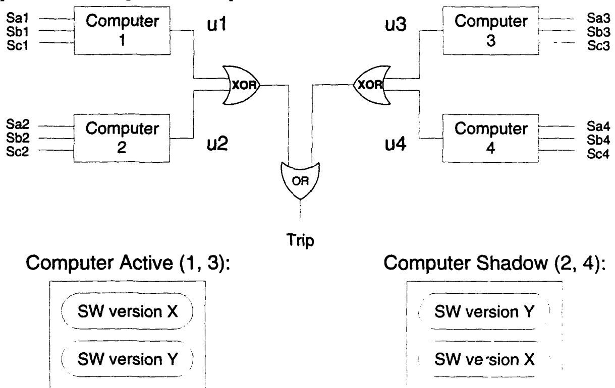
Figure B.7: Overview of the EDRB
