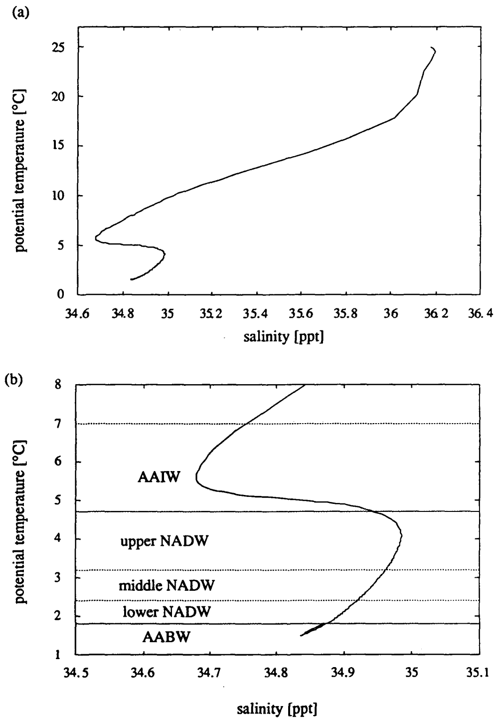
FIG. 4. A \theta -S diagram for the 11°N section, calculated by taking the average potential temperature and salinity at 20 m depth intervals, for (a) the entire water column, and (b) the isothermal boundaries defining the intermediate, deep and bottom water masses.
