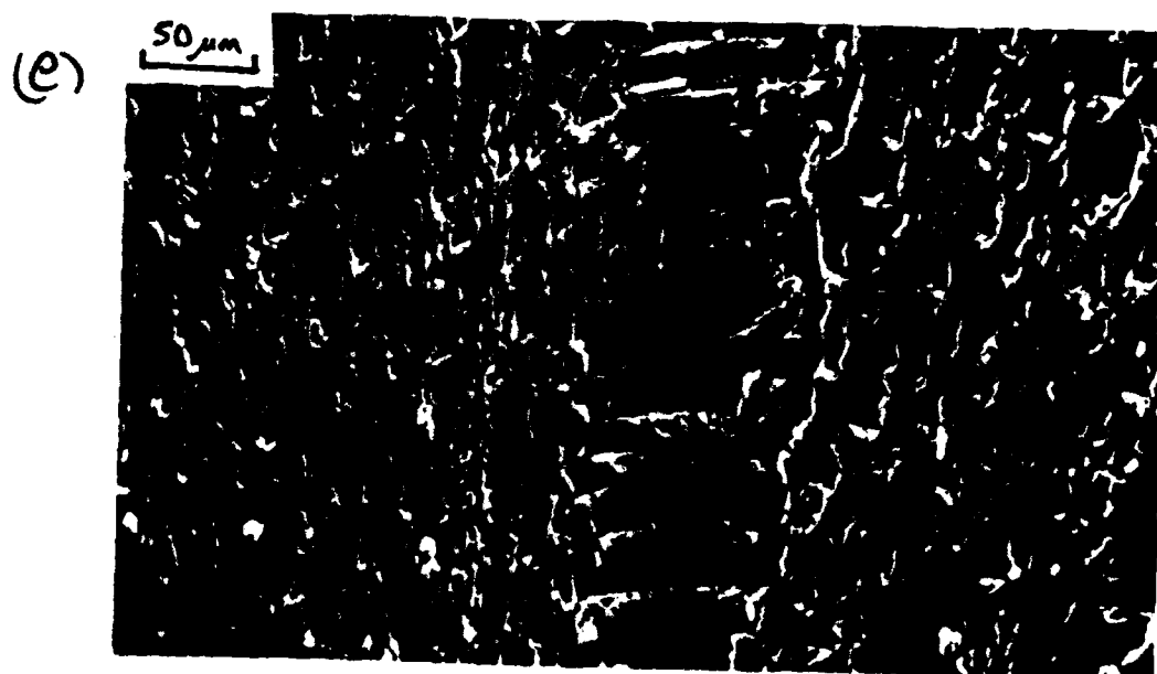
FIG.14 (Continued) (d) delaminations, splits and TPCs in the top 0/90 plies at higher load. (e) detail of splits at notch root in 0 ply.
