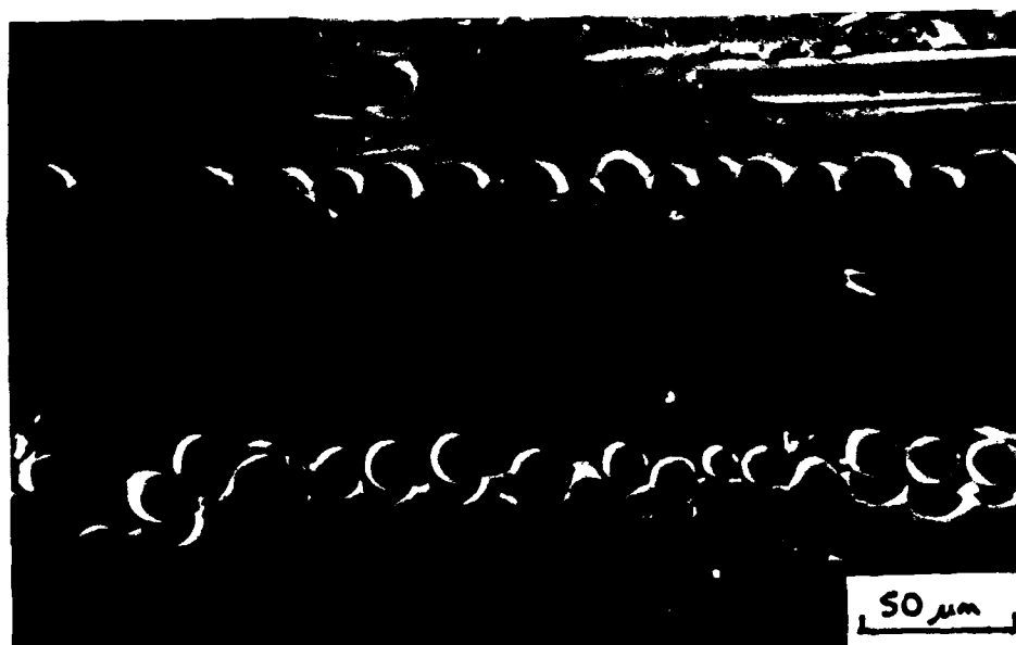
FIG.9 (Continued) (c) transverse ply crack due to tensile stress parallel to principal crack. (d) 0 ply bridging fibres exposed below the surface at greater crack opening.
