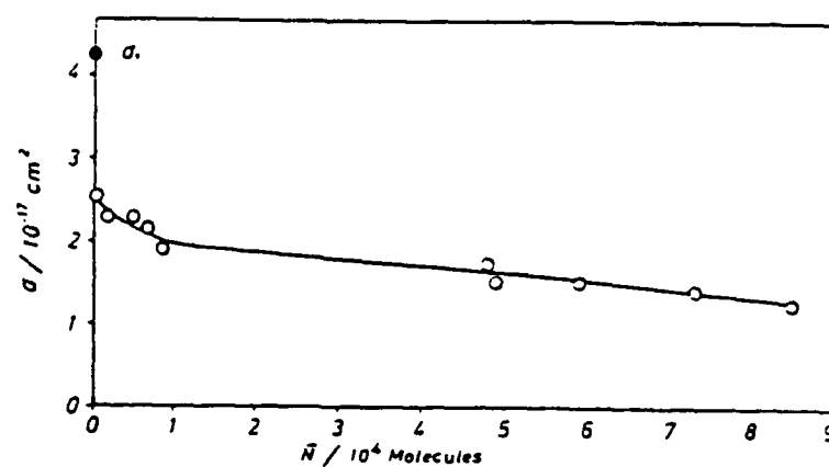
Figure 10. Effective electron impact ionization cross section of cluster beams of H_2 as a function of the mean cluster size N for 500 eV. The solid point shows the value, \sigma_1 , of the cross section for uncondensed H_2 at the same electron energy 30 .
