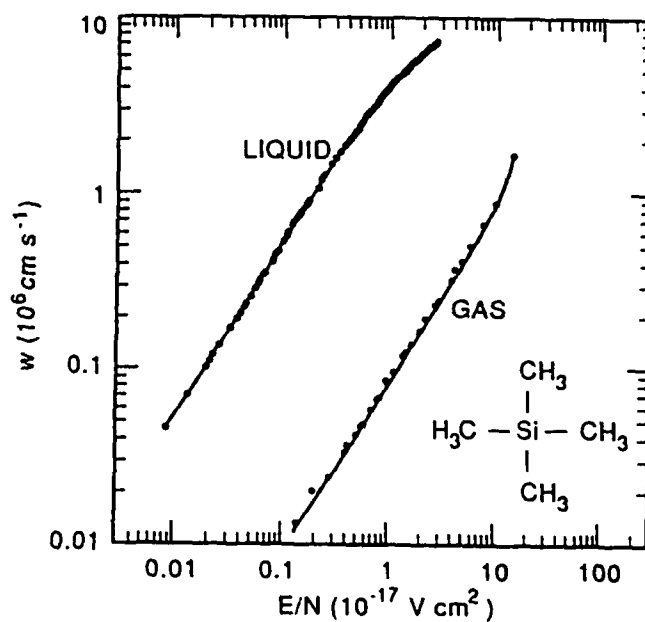
Figure 8. w vs E/N for gaseous and liquid tetramethylsilane ( T = 300 \text{ K} ) (based on Ref. 26).
