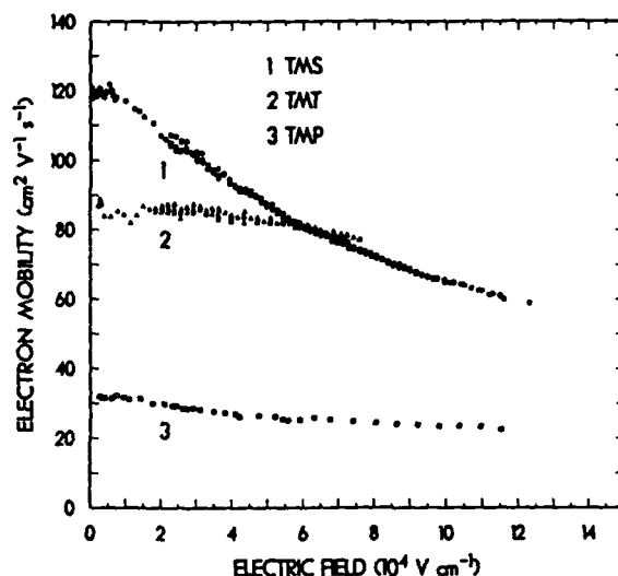
Fig. 4. Electron mobility, \mu = w/E as a function of applied electric field in neat TMS, TMT, and TMP.
