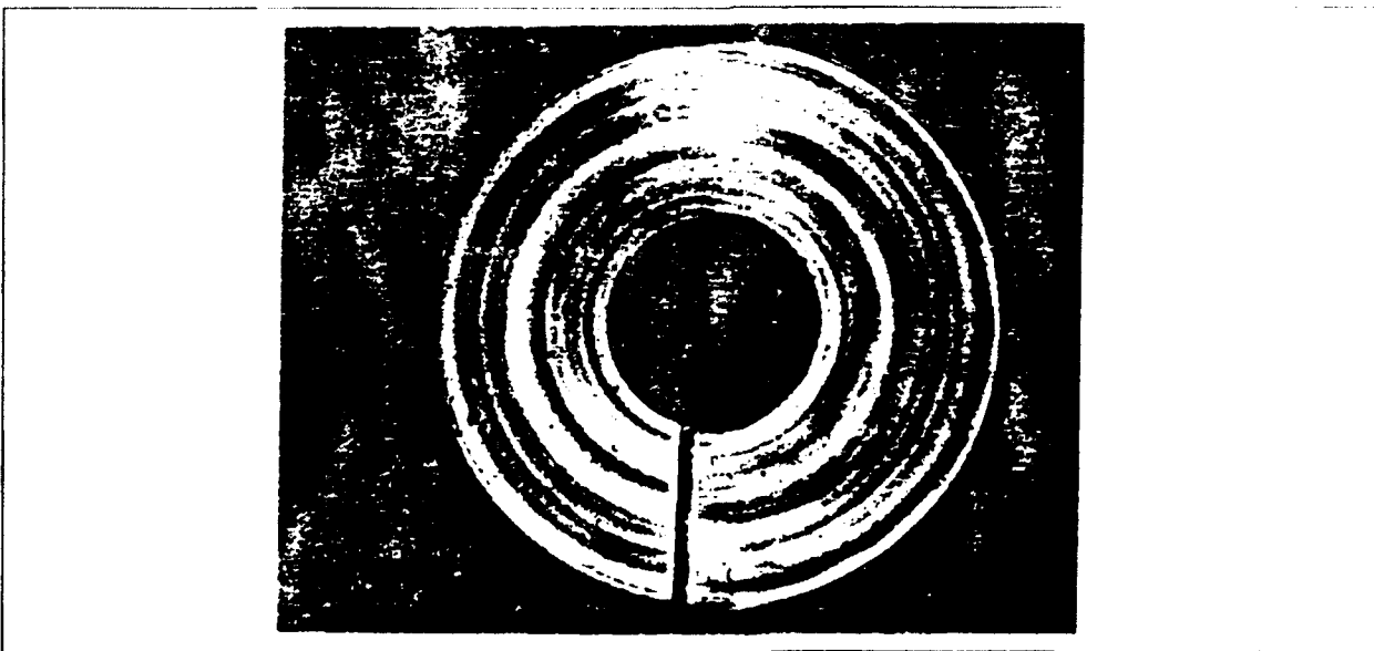
Figure 5. Knife edge photo of lens exhibiting aberrations.
