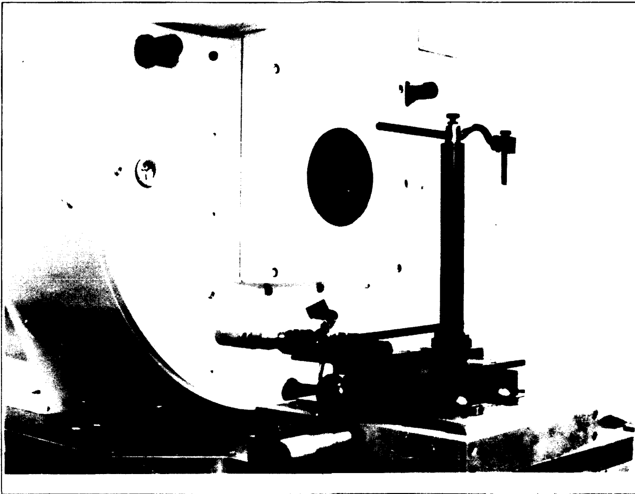
Figure 4. Knife edge behind 150-inch lens.
