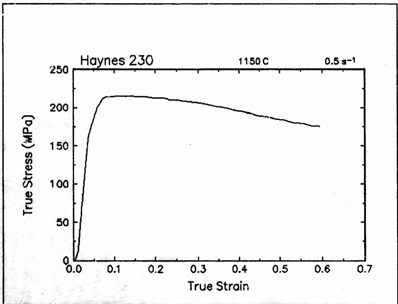
Figure 38. True stress-true strain curve, 1150 C and 0.5 s -1 .
