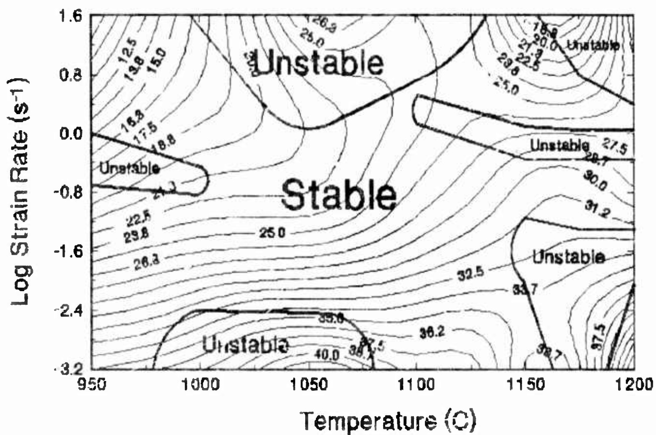
Figure 60 Processing map of Haynes 230 at a true strain of 0.30
