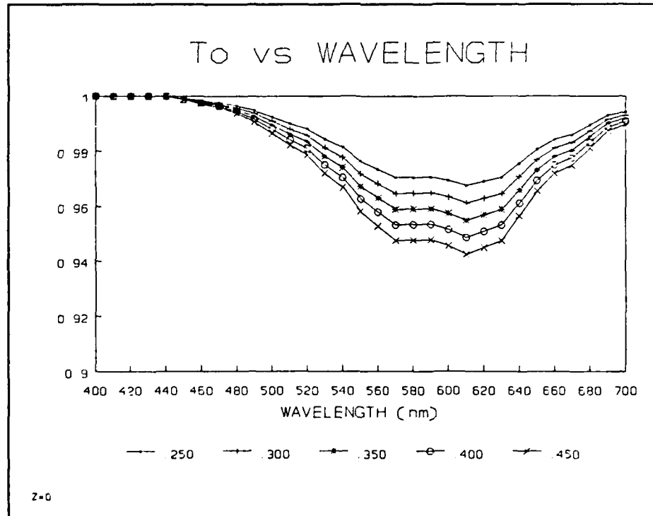
Figure 9. T_0 for a range of O_3 and a zenith angle of 0°.
