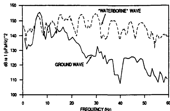
Fig. 5. Spectral energy partitioning between ground and waterborne paths.
