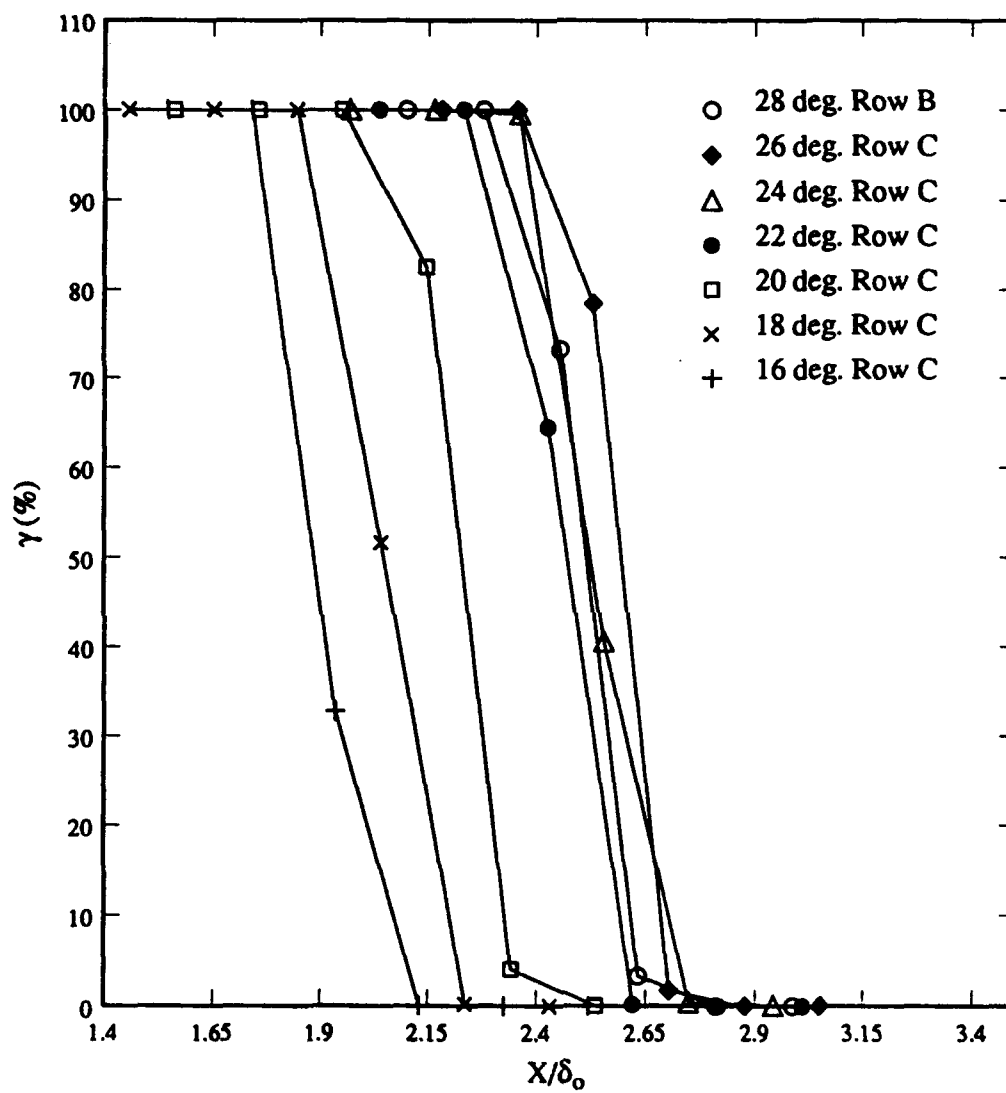
Fig. 57. Intermittency Distributions
