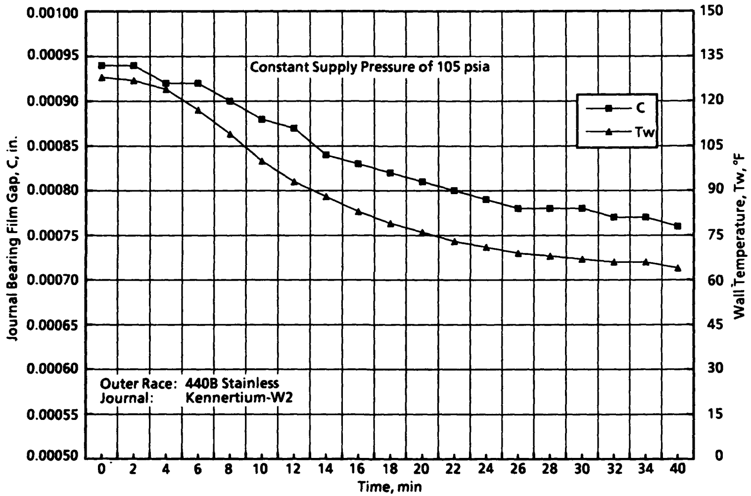
Figure 5. Thermal gradient effects to film gap.
