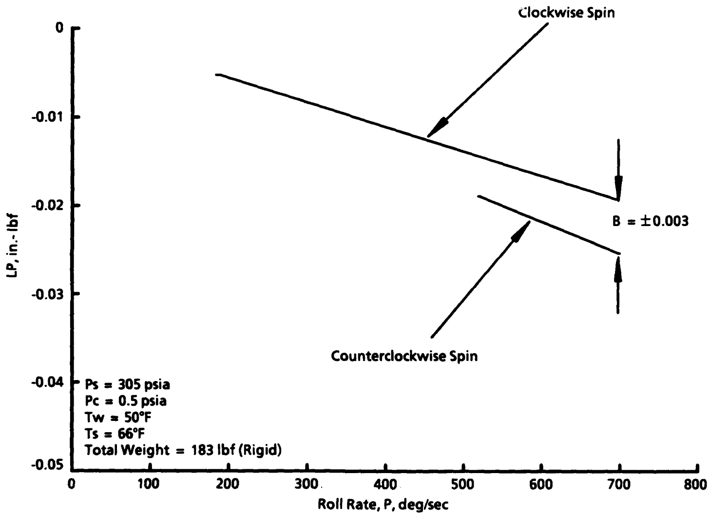
a. Viscous damping moment Figure 14. Estimation of tare bias.
