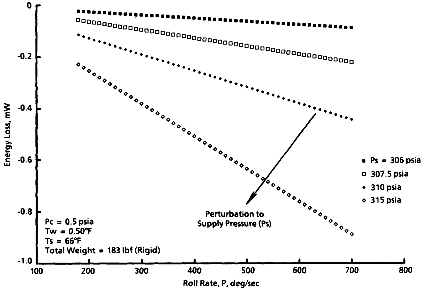
b. Supply pressure Figure 11. Continued.
