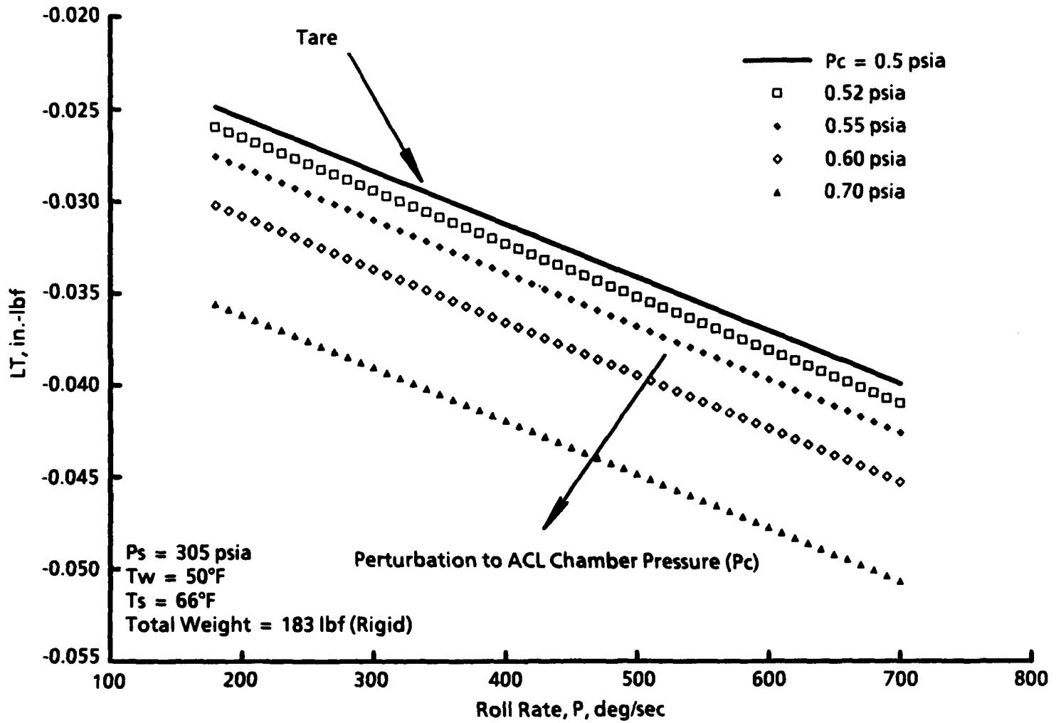
Figure 10. Tare model rolling-moment profiles for chamber pressure perturbations.
