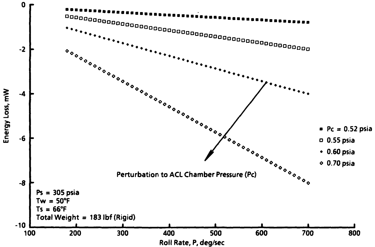
a. Chamber pressure
