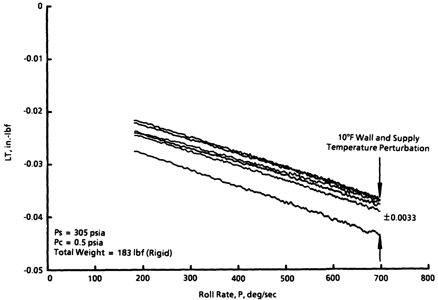
Figure 12. Application of the tare math model for temperature perturbations.
