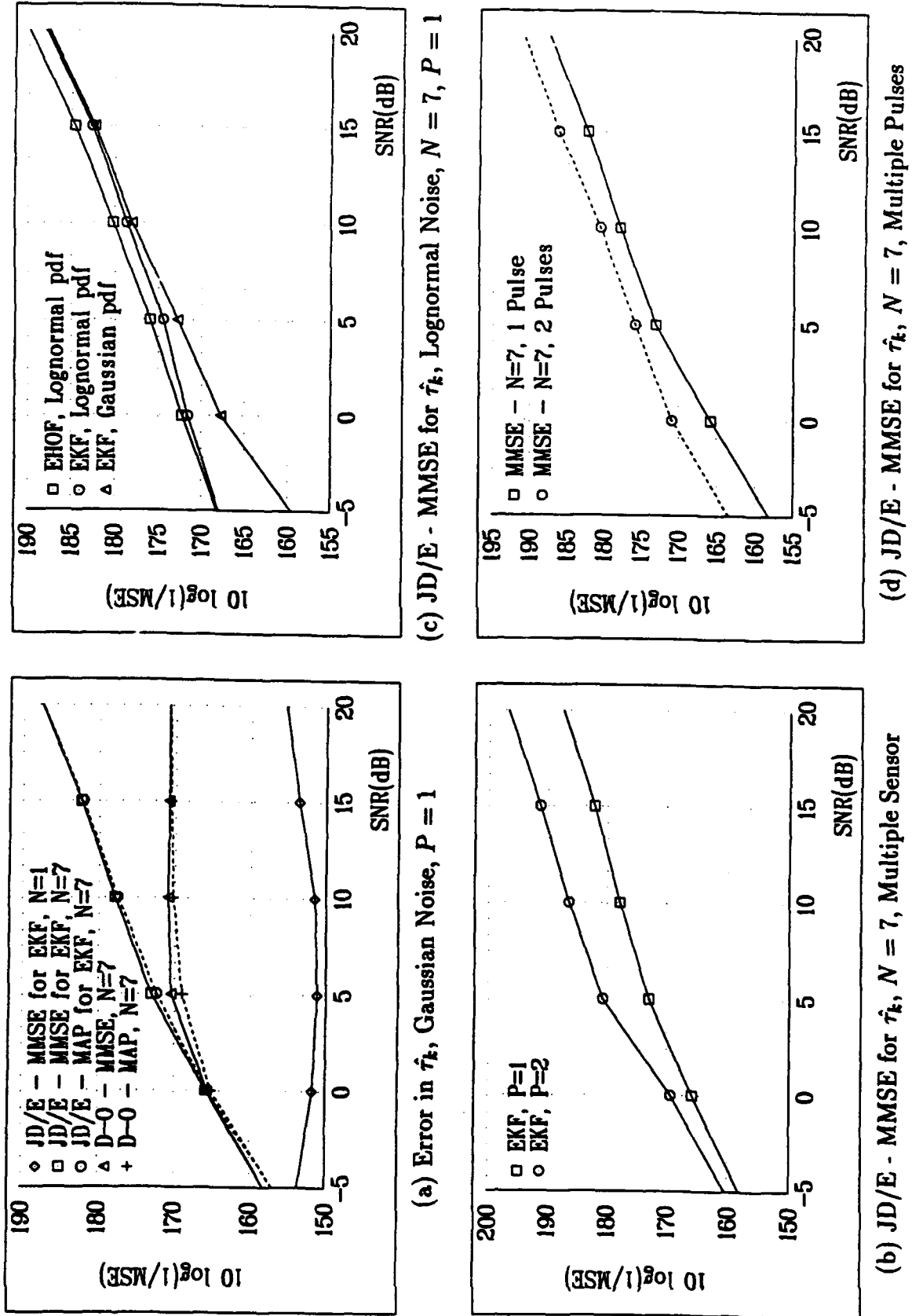
Figure 7.2 JD/E Performance for Time Delay Estimation
