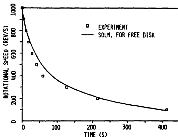
Figure 2. COASTDOWN CURVE FOR 2.5 CM ROTOR
