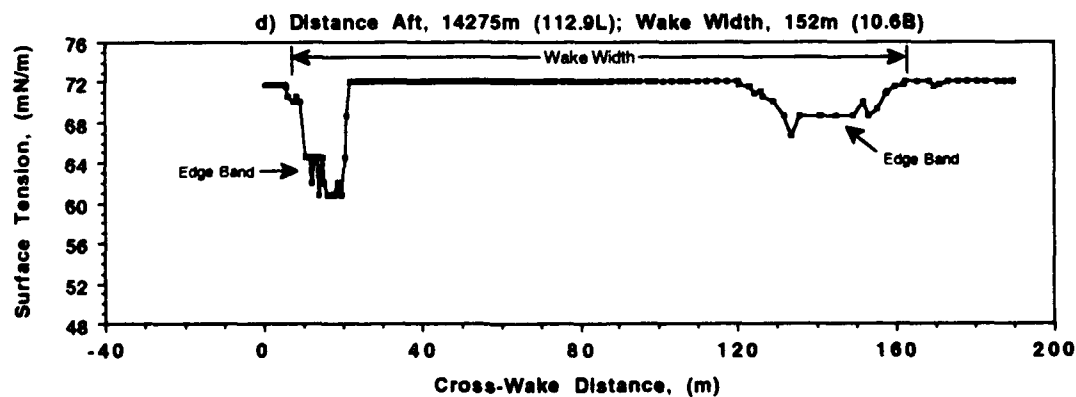
Figure 17. Measured cross-wake surface tension distribution (a) 1607, (b) 4790, (c) 9703, and (d) 14,275 m aft of the Navy frigate. The ship speed was 12 knots, or 6.2 m/s ( Fr \approx 0.176 ).
