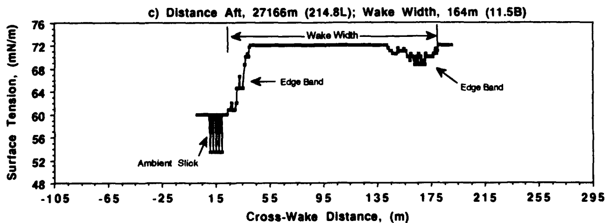
Figure 18. Measured cross-wake surface tension distribution (a) 4637, (b) 13,975, and (c) 27,166 m aft of the Navy frigate. The ship speed was 25 knots, or 12.9 m/s ( Fr = 0.366 ).
