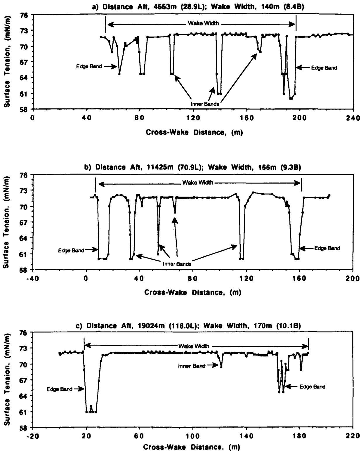
Figure 13. Measured cross-wake surface tension distribution (a) 4663, (b) 11,425, and (c) 19,024 m aft of the Navy destroyer. The ship speed was 25 knots, or 12.9 m/s ( Fr = 0.324 ).
