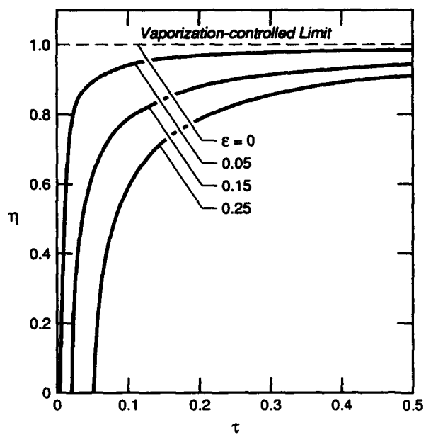
Figure 24. Melt velocity vs. time, matched asymptotic solution.
