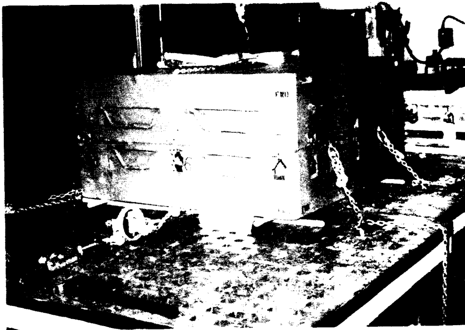
Figure 57. Freedom strength test, CN-10-1, 1000 lbs. Forward Constraint Loading of Freedom Barrels.
