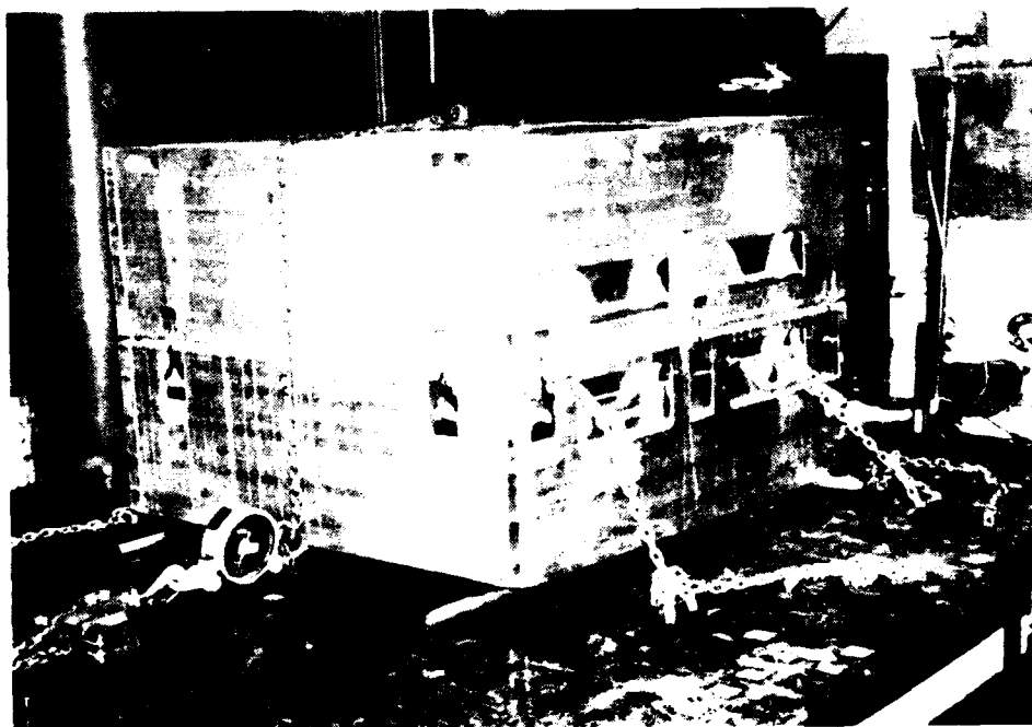
Figure 58. Freedom strength test, CN-10-1, 1000 lbs. 2 Constraint Loading, lower barrel, 1000 lbs. Failure by Buckling from Interior, 1000 lbs. of Force.
