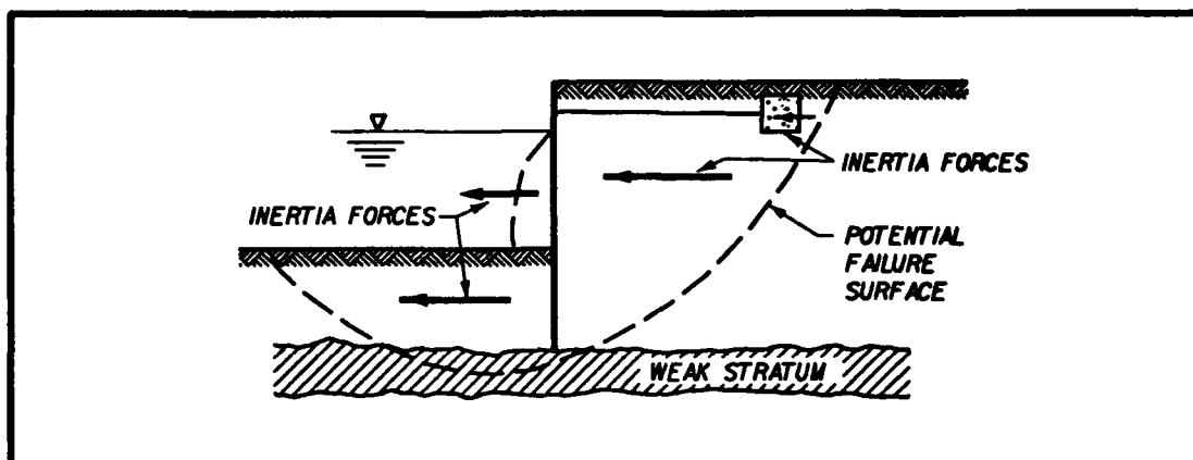
Figure 2.7 Failure surface below wall
