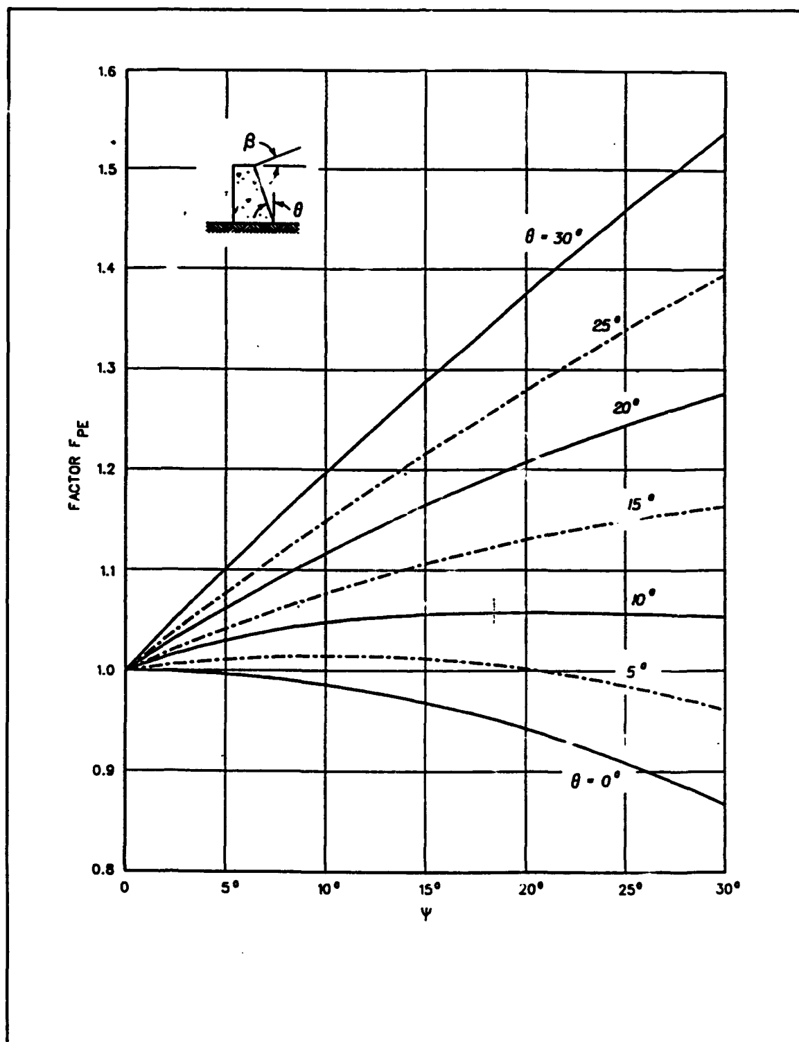
Figure 4.17 Values of factor F_{PE}
