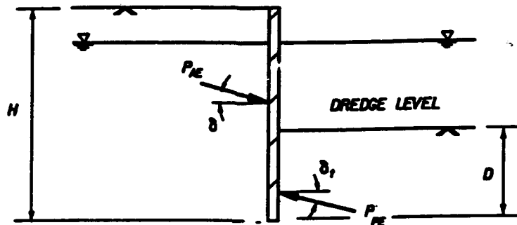
(a.) Mononobe - Okabe Earth Pressure Forces P_{AE} and P_{FE} .
