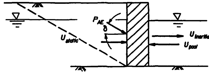
CASE 2: Submerged BackFill, No Excess Pore Water Pressures Due to Earthquake.
