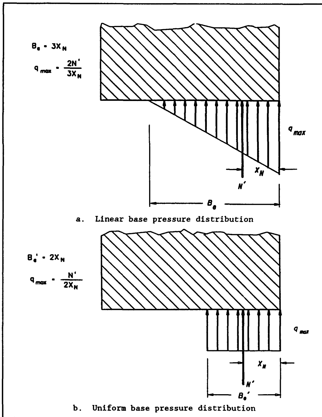
Figure 6.3 Linear and uniform base pressure distributions
