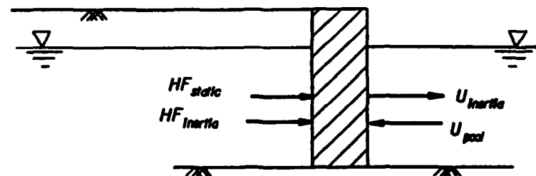
CASE 4: Liquefied BackFill.
