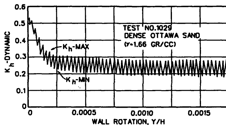
(b). Dynamic Horizontal Earth Pressure
