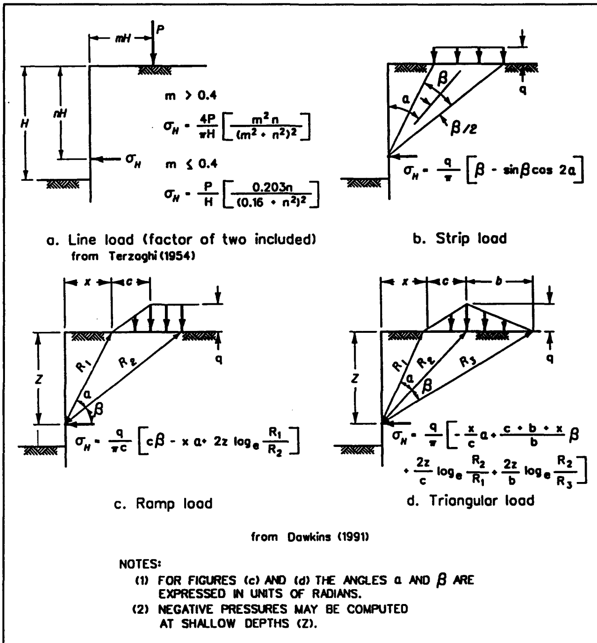
Figure 3.13 Theory of elasticity equations for pressures on wall due to surcharge loads
