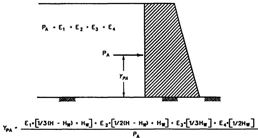
d. Resultant effective force and point of application
