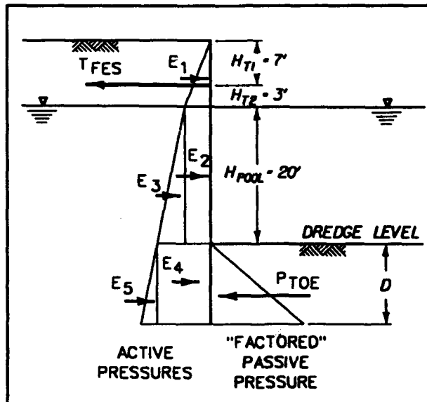
Figure C.2 Horizontal earth pressure components in free earth support design
