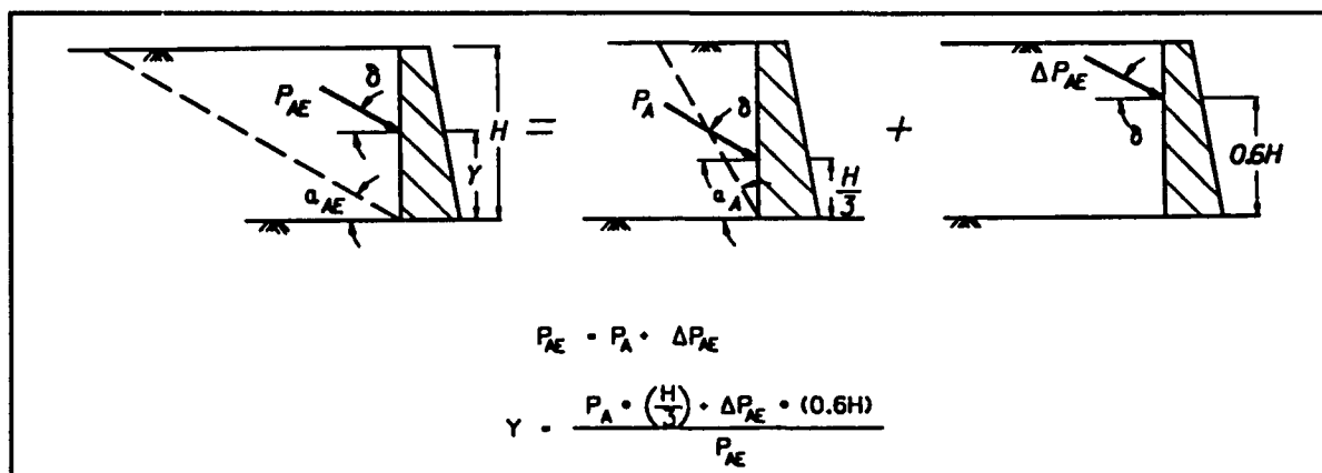
Figure 4.10 Static active earth pressure force and incremental dynamic active earth pressure force for dry backfill
