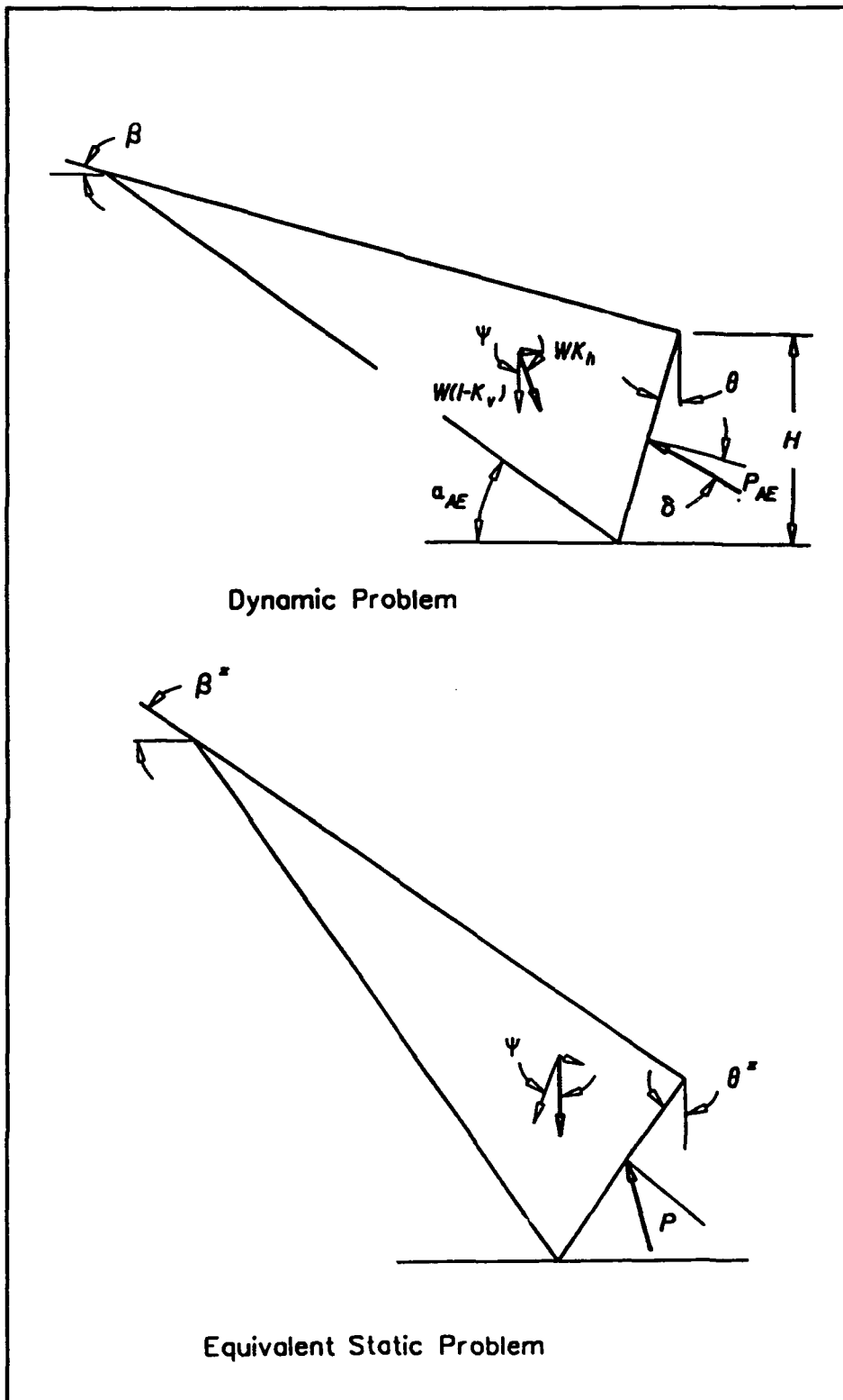
Figure 4.7 Equivalent static formulation of the Mononobe-Okabe active dynamic earth pressure problem
