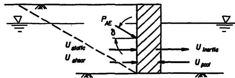
CASE 3: Submerged BackFill, Excess Pore Water Pressures Due to Earthquake.
