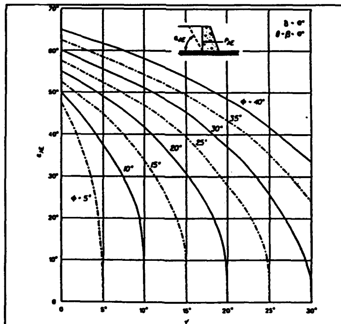
Figure 4.5 Variation in \alpha_{AE} with \phi for \delta equal to zero degrees, vertical wall and level backfill
