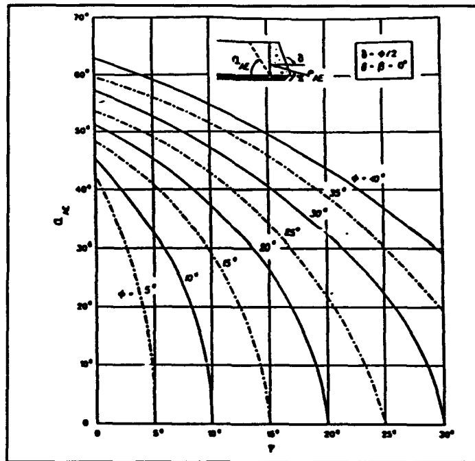
Figure 4.4 Variation in \alpha_{AE} with \phi for \delta equal to \phi/2 , vertical wall and level backfill
