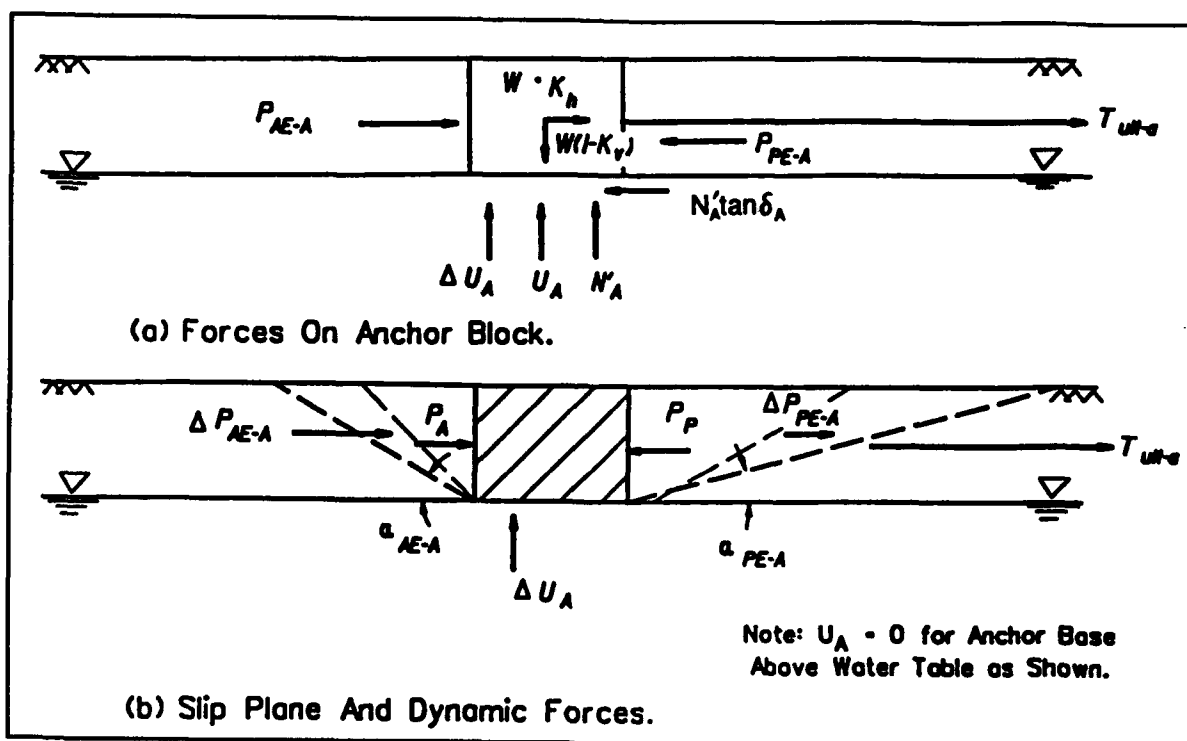
Figure 7.11 Dynamic forces acting on an anchor block (for \delta = 0^\circ )
