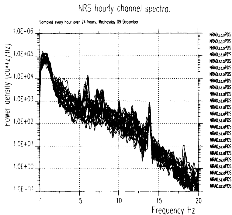
Fig. 7.2.2b. Same as Fig. 7.2.2a but for NORESS data (A0 SPZ seismometer) taken hourly between 00.00 and 23.00 hours GMT on day 344, 1992.
