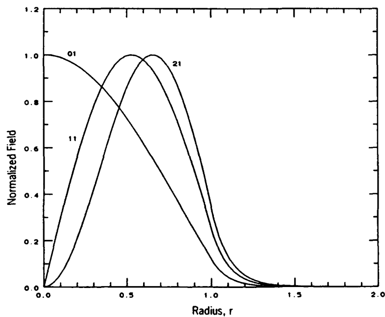
Fig. 10. Field patterns for the LP 01 , LP 11 , and LP 21 modes of a step index fiber with \Delta=0.038 . These patterns were computed using R_{\text{fiber}}=10R_{\text{core}} , V=10 , and 32 points in the core.
