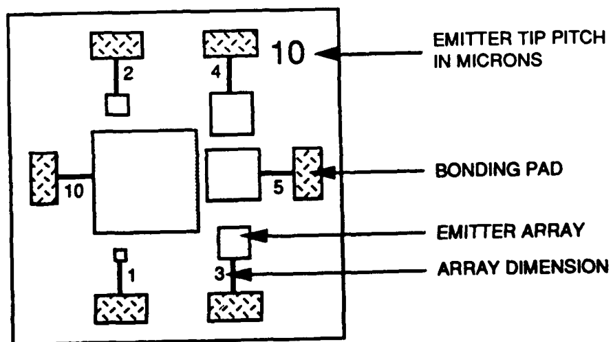
Figure 13. Arrays for per-tip current studies.
