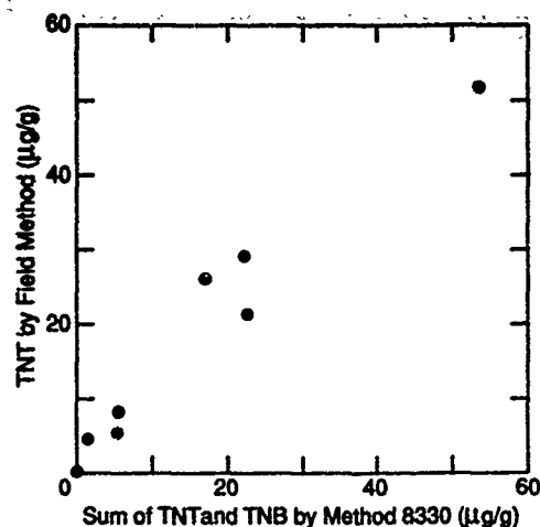
Figure 3. Correlation of estimates of TNT concentration obtained by the field method with those obtained by Method 8330 ( y = 1.03x + 0.39 , R^2 = 0.98 ).
