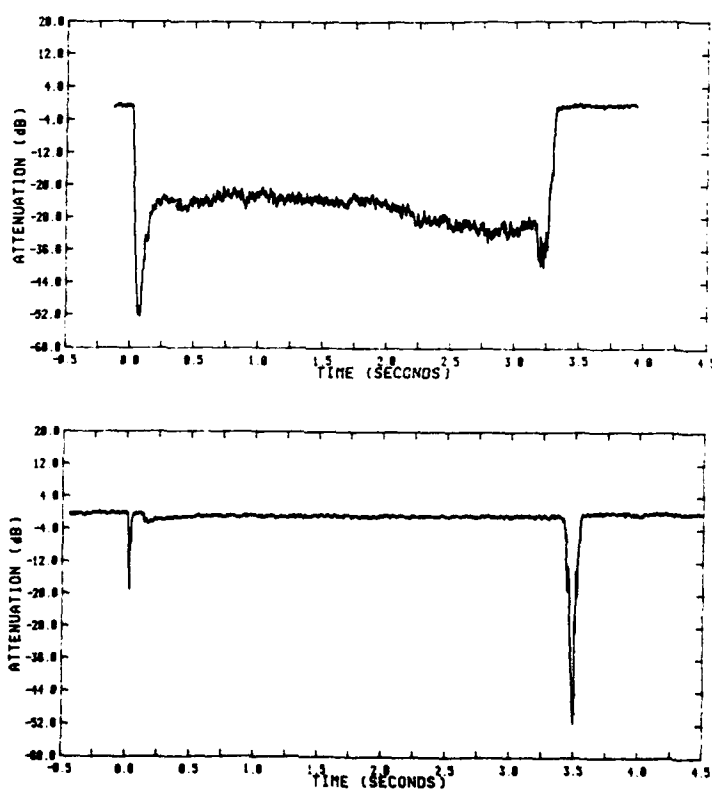
Figure 18 Millimetric Wave Radar Attenuation (30° to plume)
