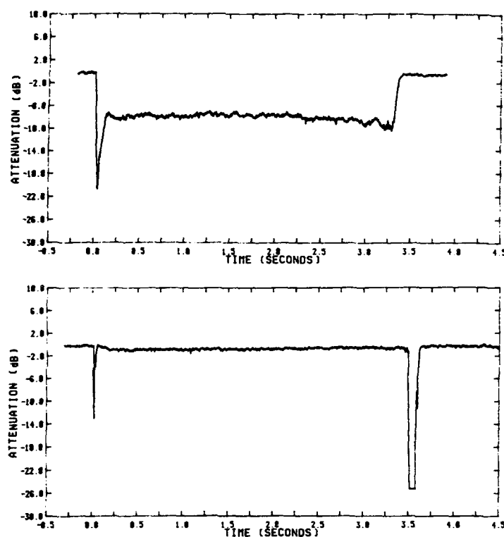
Figure 17 Millimetric Wave Radar Attenuation (Normal to plume)
