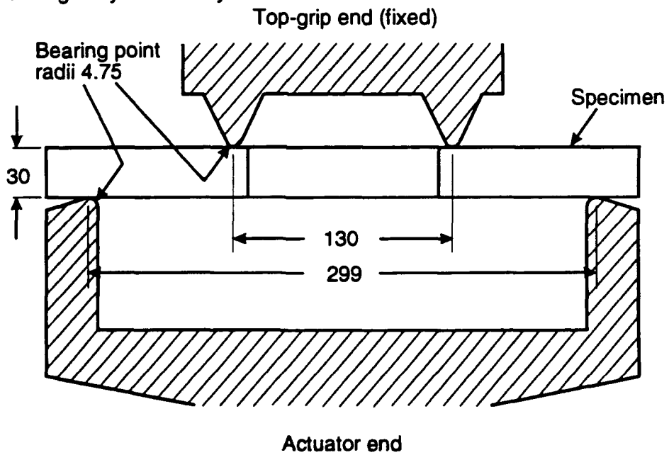
(b) Test jig
